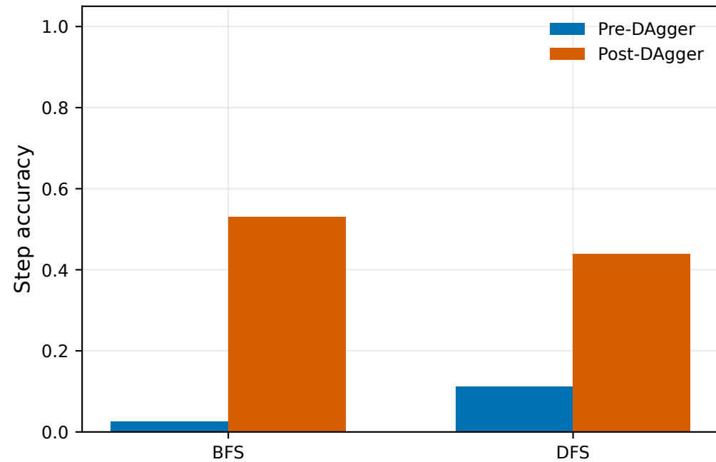
Main-task accuracy
