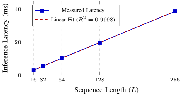
Fig. 5. Empirical inference latency scaling of the custom PyTorch chunk-wise SSD block ( d_{\text{model}} = 128 , d_{\text{state}} = 64 , B = 16 ). Measurements exhibit approximately linear empirical latency scaling over the tested sequence lengths.
