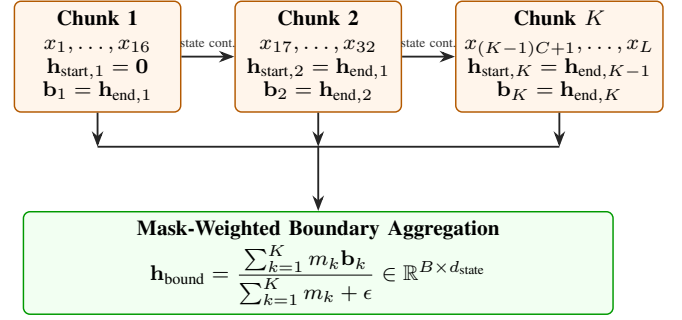
Fig. 3. State-continuous chunk-wise SSD-style recurrence with boundary state extraction. Recurrent hidden states propagate continuously across chunk boundaries ( \mathbf{h}_{\text{start},k} = \mathbf{h}_{\text{end},k-1} ) with zero state resets, while mask-weighted aggregation prevents zero-padding bias.
