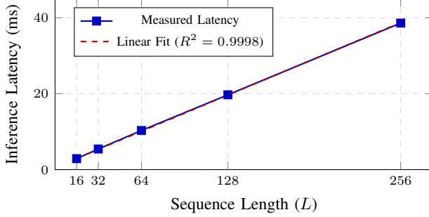
Fig. 5. Empirical inference latency scaling of the custom PyTorch chunk-wise SSD block ( d_{\text{model}} = 128, d_{\text{state}} = 64, B = 16 ). Measurements exhibit approximately linear empirical latency scaling over the tested sequence lengths.
