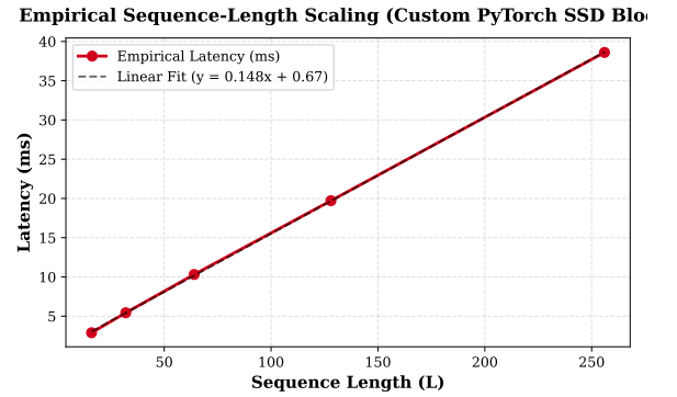
Fig. 3: Empirical inference latency scaling of custom PyTorch chunk-wise SSD block ( d_{\text{model}} = 128, d_{\text{state}} = 64, B = 16 ). Measurements confirm linear scaling \mathcal{O}(L) .
