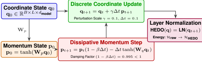
Fig. 3. Computational flow of the Hamiltonian-Inspired Energy Dissipation Operator (HEDO). Coordinate representations \mathbf{q}_0 initialize conjugate momenta \mathbf{p}_0 . Discrete updates execute damped momentum updates ((1 - \beta\Delta t) = 0.995) and discrete coordinate updates before Layer Normalization.
