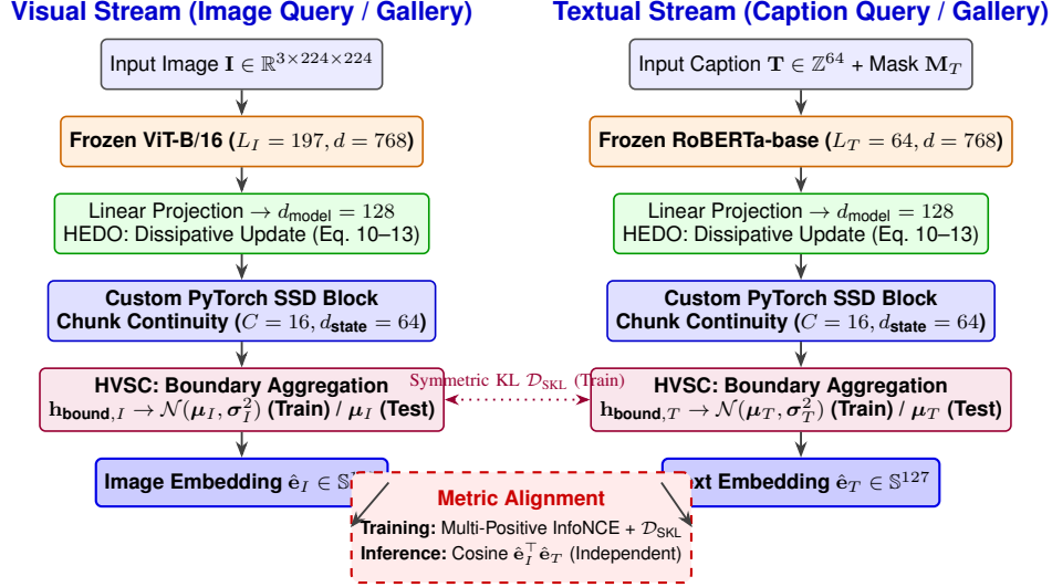
Fig. 1. Overall architectural pipeline of the proposed HEDO-HVSC multimodal state-space framework. Visual patch sequences ( L_I = 197 ) and textual token sequences ( L_T = 64 ) are extracted from frozen ViT-B/16 and RoBERTa-base encoders, projected to d_{\text{model}} = 128 , stabilized via HEDO coordinate-momentum dissipation, and processed through custom chunk-wise SSD recurrence blocks ( C = 16, d_{\text{state}} = 64 ). During training, mask-weighted boundary states parameterize Gaussian latent distributions regularized via symmetric KL divergence \mathcal{D}_{\text{SKL}} alongside multi-positive InfoNCE contrastive alignment. At test time, retrieval evaluates deterministic posterior means strictly unimodally with zero cross-modal communication.
