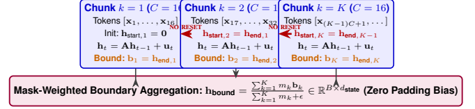
Fig. 4. State-continuous chunk-wise SSD-style recurrence with boundary state extraction. Recurrent hidden states propagate continuously across chunk boundaries ( \mathbf{h}_{\text{start}, k} = \mathbf{h}_{\text{end}, k-1} ) with zero state resets, while mask-weighted aggregation prevents zero-padding bias.
