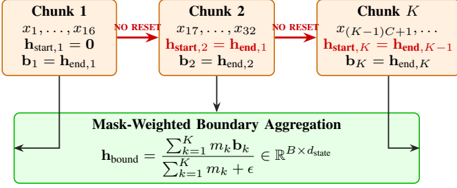
Fig. 3. State-continuous chunk-wise SSD-style recurrence with boundary state extraction. Recurrent hidden states propagate continuously across chunk boundaries ( \mathbf{h}_{\text{start},k} = \mathbf{h}_{\text{end},k-1} ) with zero state resets, while mask-weighted aggregation prevents zero-padding bias.
