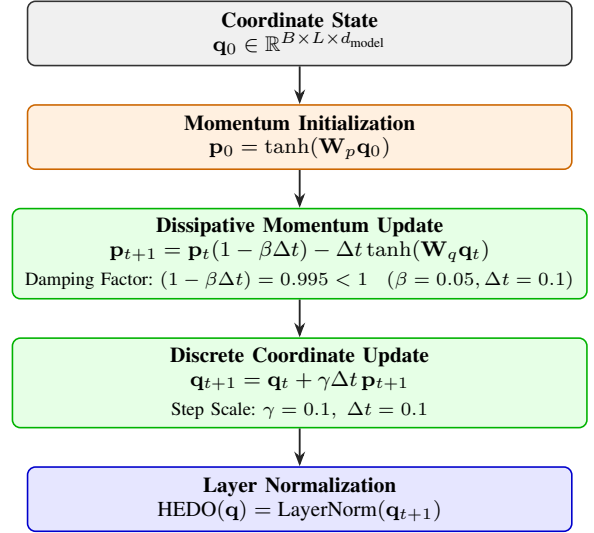
Fig. 2. Computational flow of the Hamiltonian-Inspired Energy Dissipation Operator (HEDO). Coordinate representations \mathbf{q}_0 initialize conjugate momenta \mathbf{p}_0 . Discrete updates execute damped momentum updates ((1 - \beta\Delta t) = 0.995) and discrete coordinate updates before Layer Normalization.
