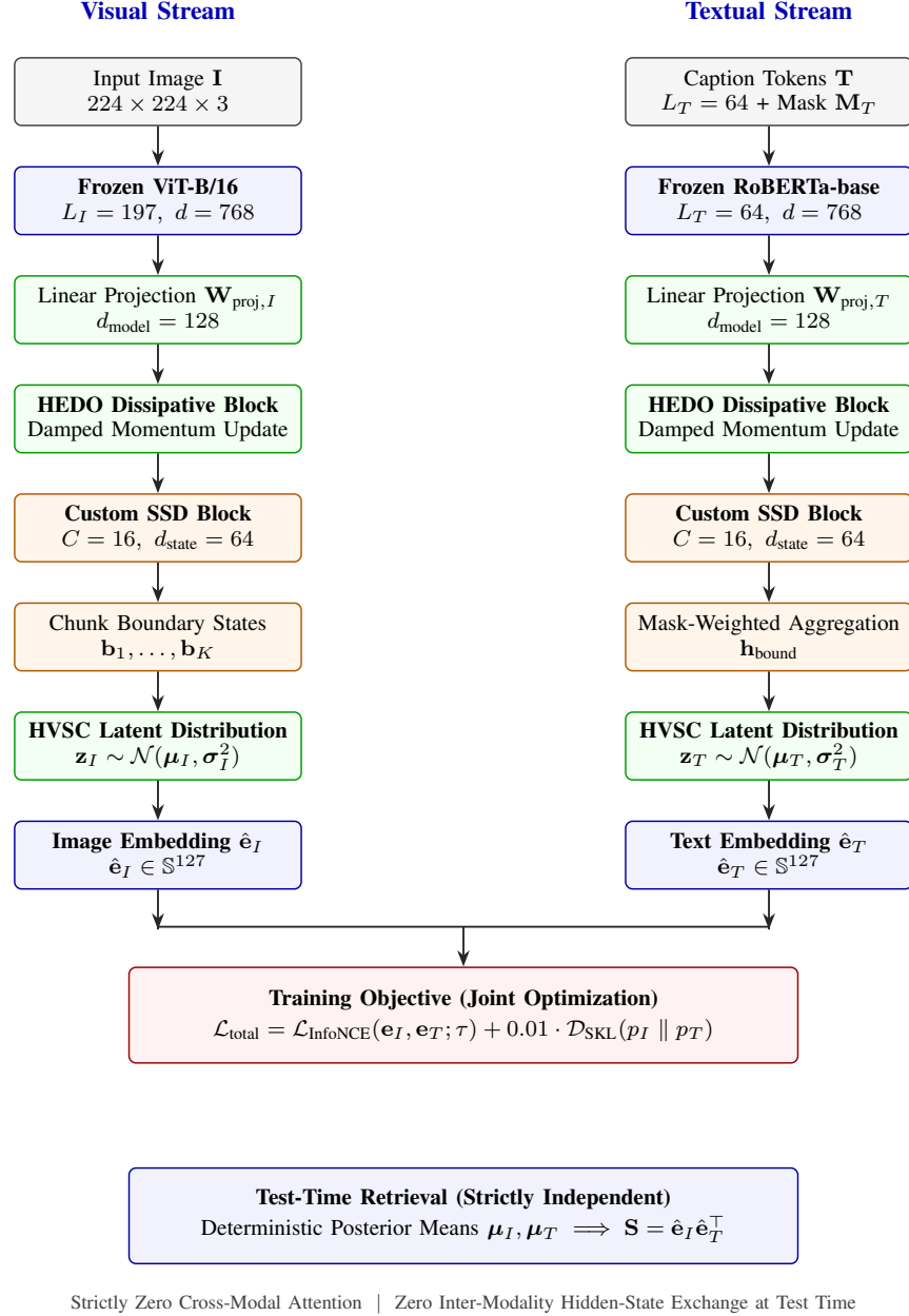
Fig. 1. Overall architectural pipeline of the proposed HEDO-HVSC multimodal state-space framework. Visual patch sequences ( L_I = 197 ) and textual token sequences ( L_T = 64 ) are extracted from frozen ViT-B/16 and RoBERTa-base encoders, projected to d_{\text{model}} = 128 , stabilized via HEDO coordinate-momentum dissipation, and processed through custom chunk-wise SSD recurrence blocks ( C = 16, d_{\text{state}} = 64 ). During training, mask-weighted boundary states parameterize Gaussian latent distributions regularized via symmetric KL divergence \mathcal{D}_{\text{SKL}} alongside multi-positive InfoNCE contrastive alignment. At test time, retrieval evaluates deterministic posterior means strictly unimodally with zero cross-modal communication.
