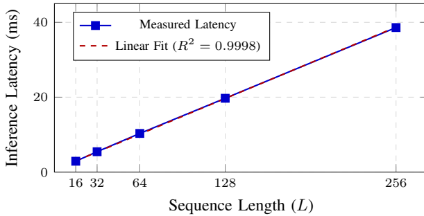
Fig. 8. Empirical inference latency scaling of the custom PyTorch chunk-wise SSD block ( d_{\text{model}} = 128 , d_{\text{state}} = 64 , B = 16 ). Measurements exhibit approximately linear empirical latency scaling over the tested sequence lengths.
