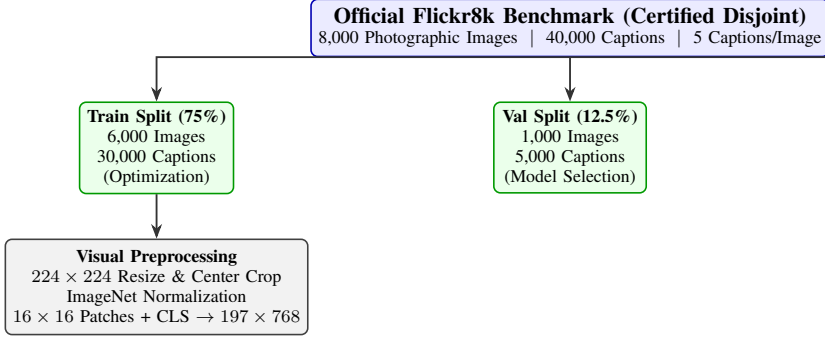
Fig. 2. Official Flickr8k dataset partition and modality-specific feature extraction pipeline. The 8,000 photographic images and 40,000 human-annotated captions are partitioned into verified disjoint training (6,000), validation (1,000), and held-out test (1,000) splits with zero cross-split leakage.
