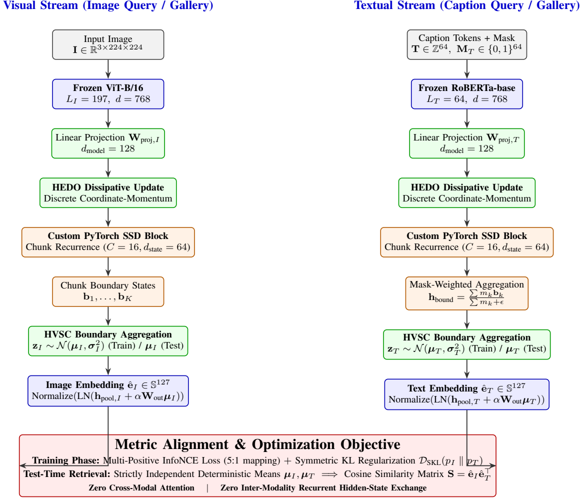
Fig. 1. Overall architectural pipeline of the proposed HEDO-HVSC multimodal state-space framework. Visual patch sequences ( L_I = 197 ) and textual token sequences ( L_T = 64 ) are extracted from frozen ViT-B/16 and RoBERTa-base encoders, projected to d_{\text{model}} = 128 , stabilized via HEDO coordinate-momentum dissipation, and processed through custom chunk-wise SSD recurrence blocks ( C = 16, d_{\text{state}} = 64 ). During training, mask-weighted boundary states parameterize Gaussian latent distributions regularized via symmetric KL divergence \mathcal{D}_{\text{SKL}} alongside multi-positive InfoNCE contrastive alignment. At test time, retrieval evaluates deterministic posterior means strictly unimodally with zero cross-modal communication.
