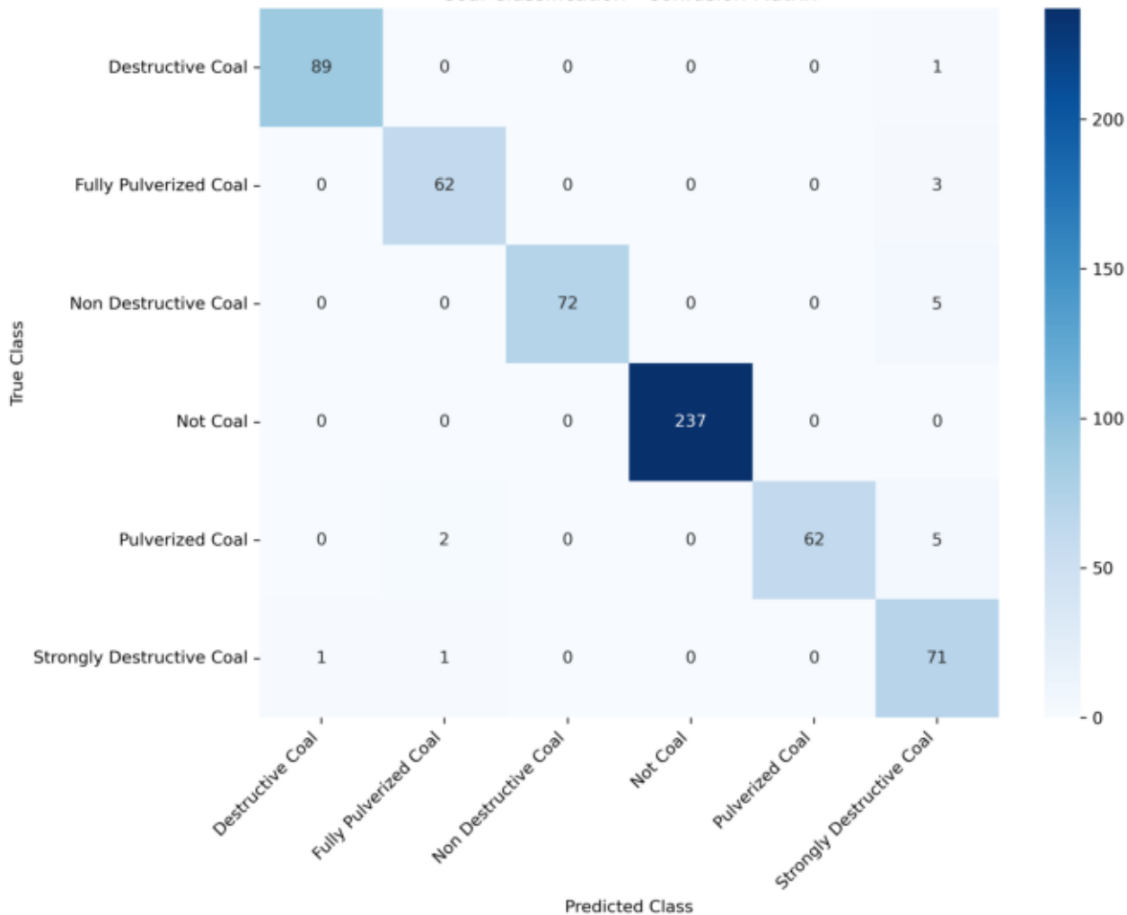
Coal Classification - Confusion Matrix
