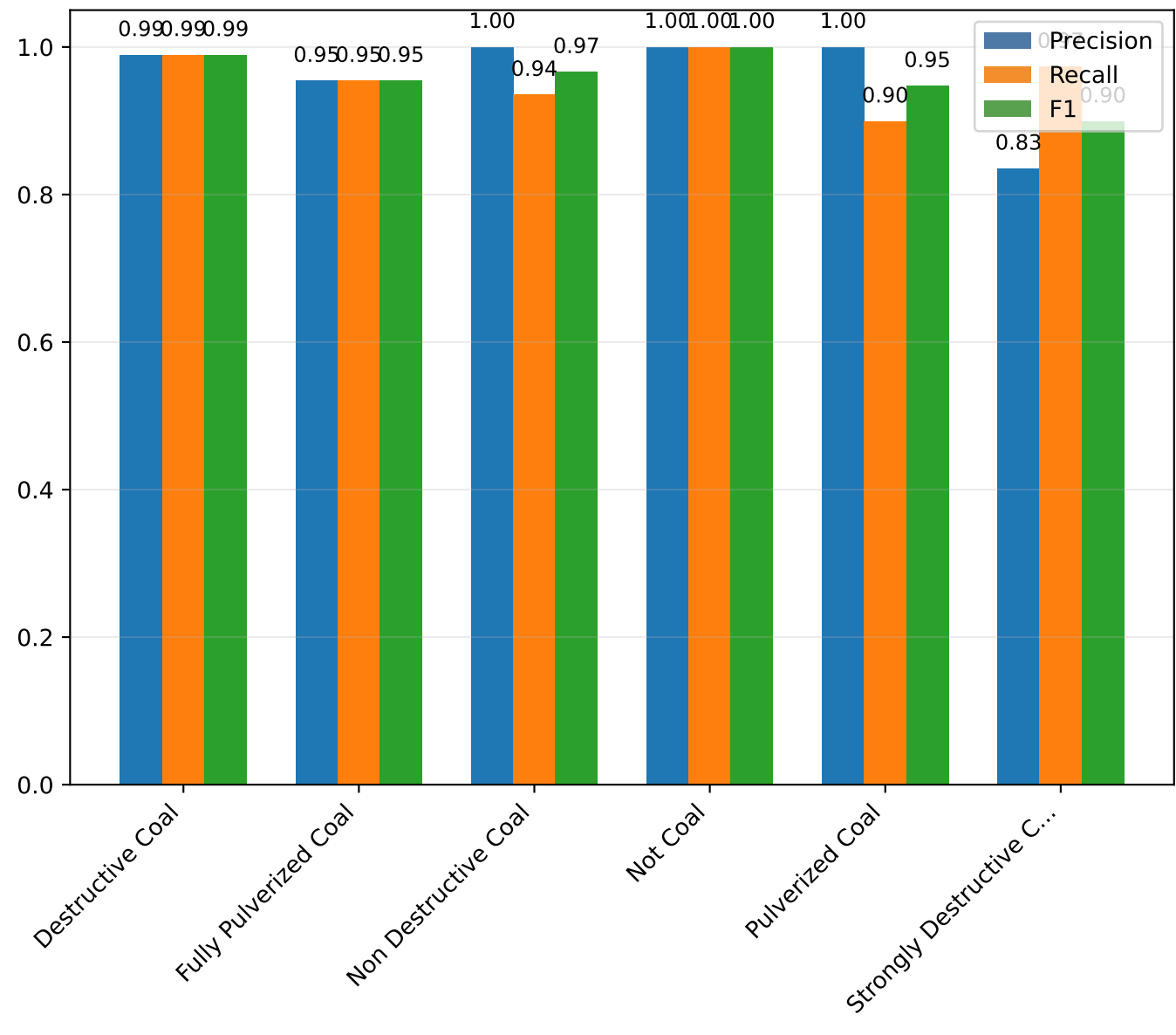
Per-class Metrics
