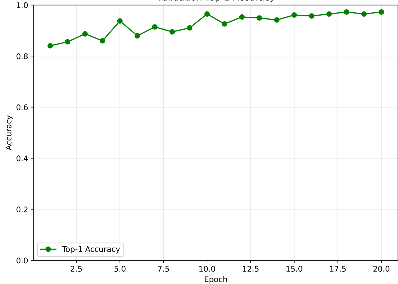
Validation Top-1 Accuracy
