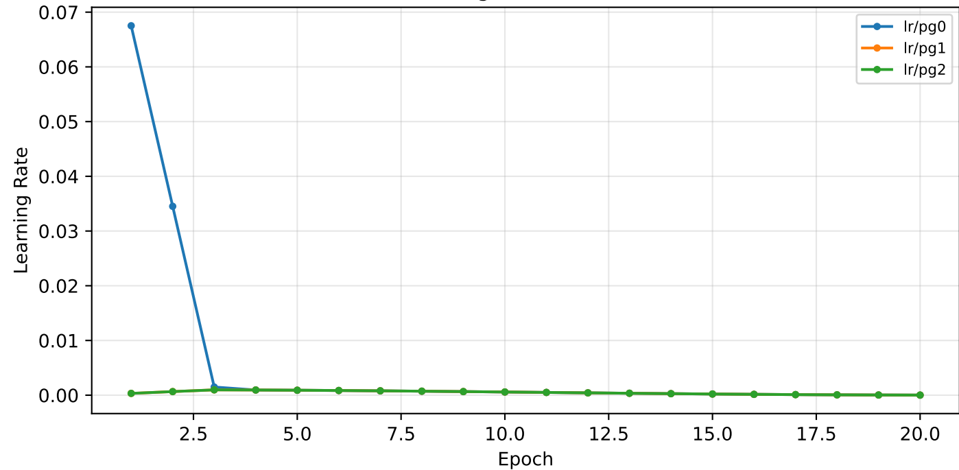
Learning Rate Schedule
