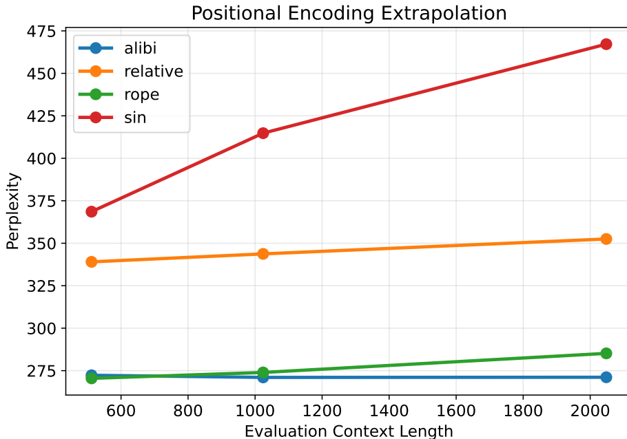
Figure 2: Perplexity as a function of evaluation context length for positional encoding methods trained at sequence length 512. ALiBi exhibits near-constant performance under extrapolation, because its distance-based penalty adjustment extends naturally beyond the training sequence length. RoPE and relative positional embeddings only show mild degradation, with the relative embeddings being helped by distance based clipping. Sinusoidal positional encoding degrades substantially at longer contexts because the model is evaluated on positional patterns beyond those seen during training, and it is unable to generalize.
