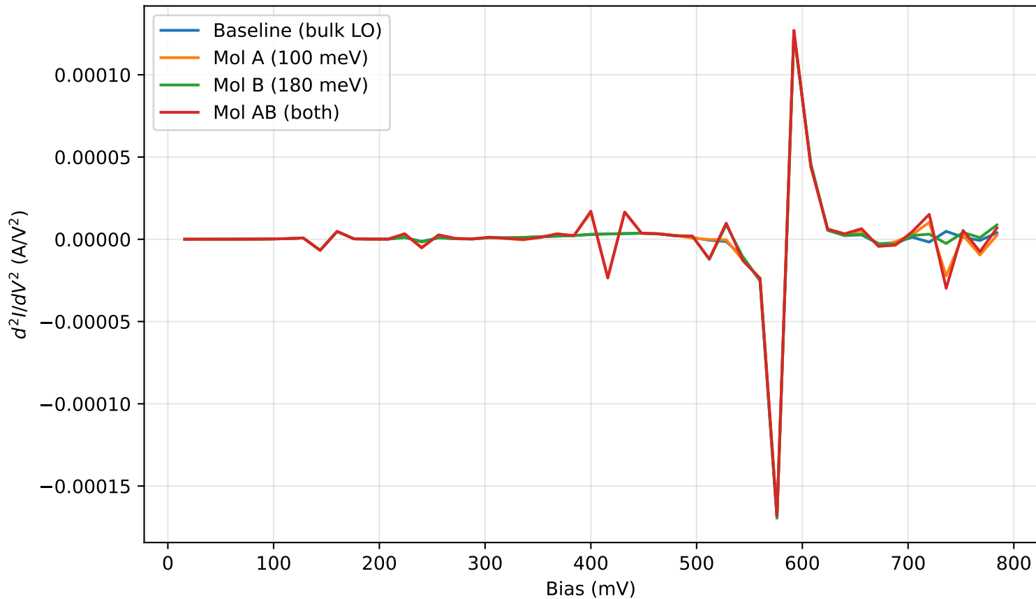
Numerical d^2I/dV^2 at 300 K (SCBA)
