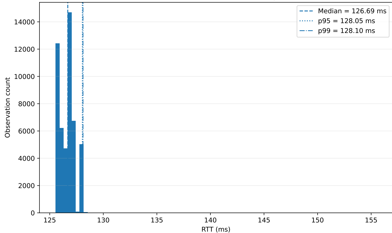
RTT Distribution: Mumbai → Tokyo
