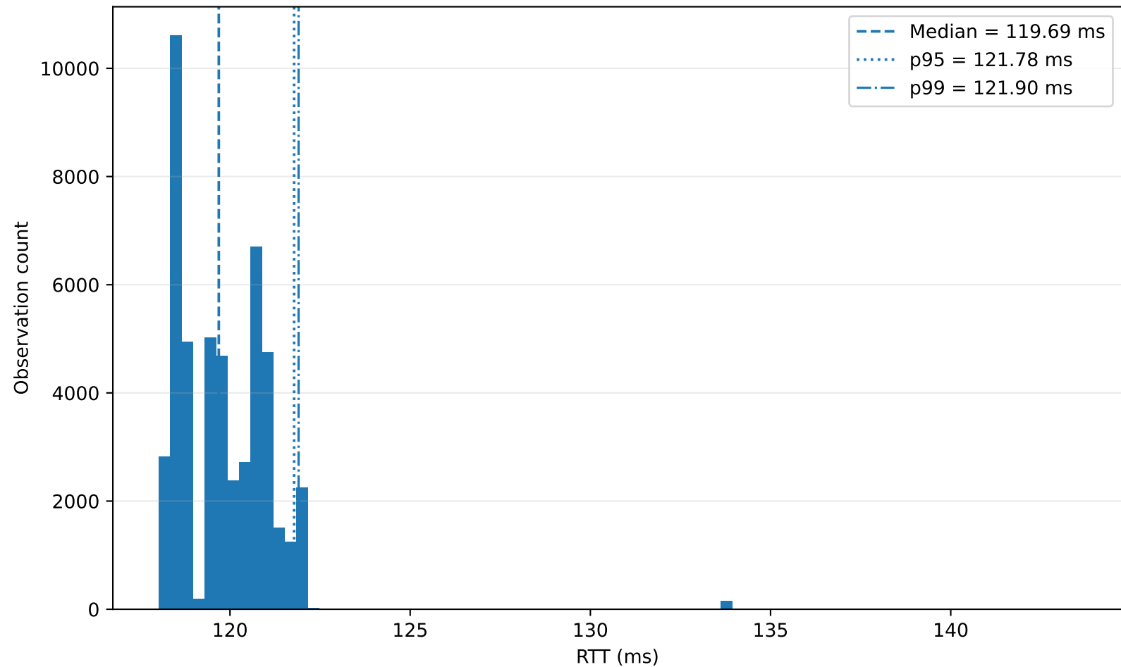
RTT Distribution: Mumbai → Ireland
