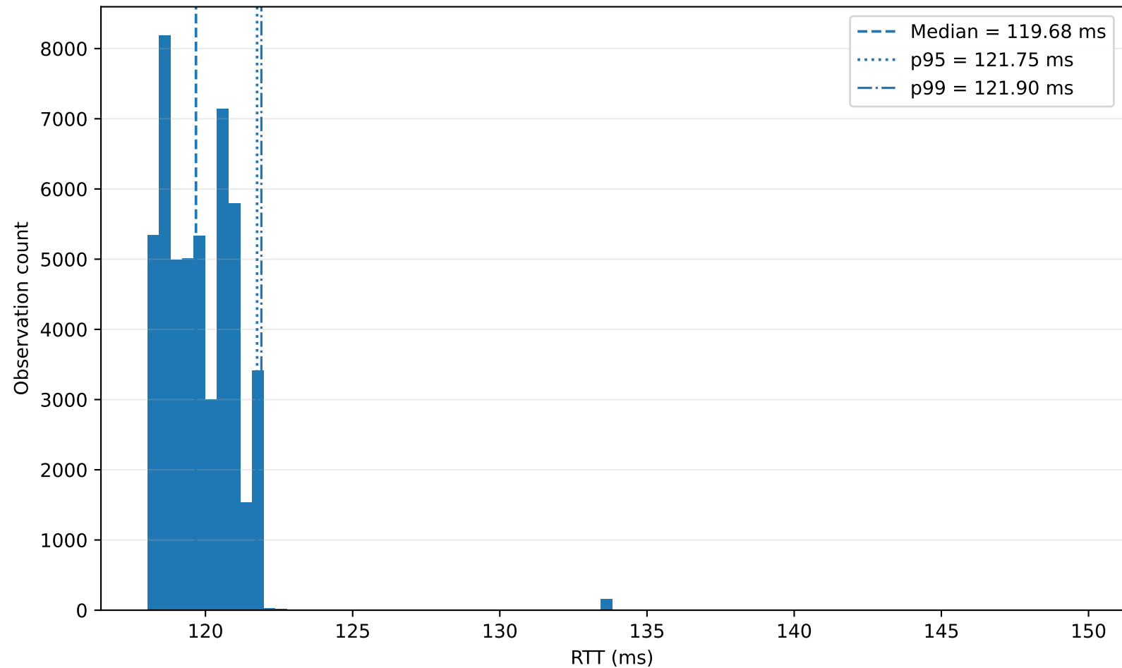
RTT Distribution: Ireland → Mumbai
