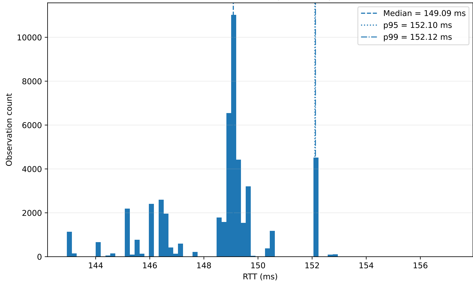
RTT Distribution: Virginia → Tokyo
