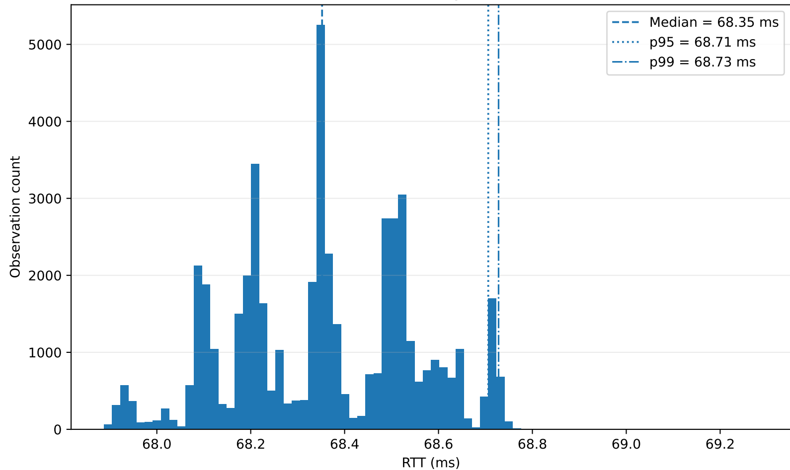
RTT Distribution: Virginia → Ireland
