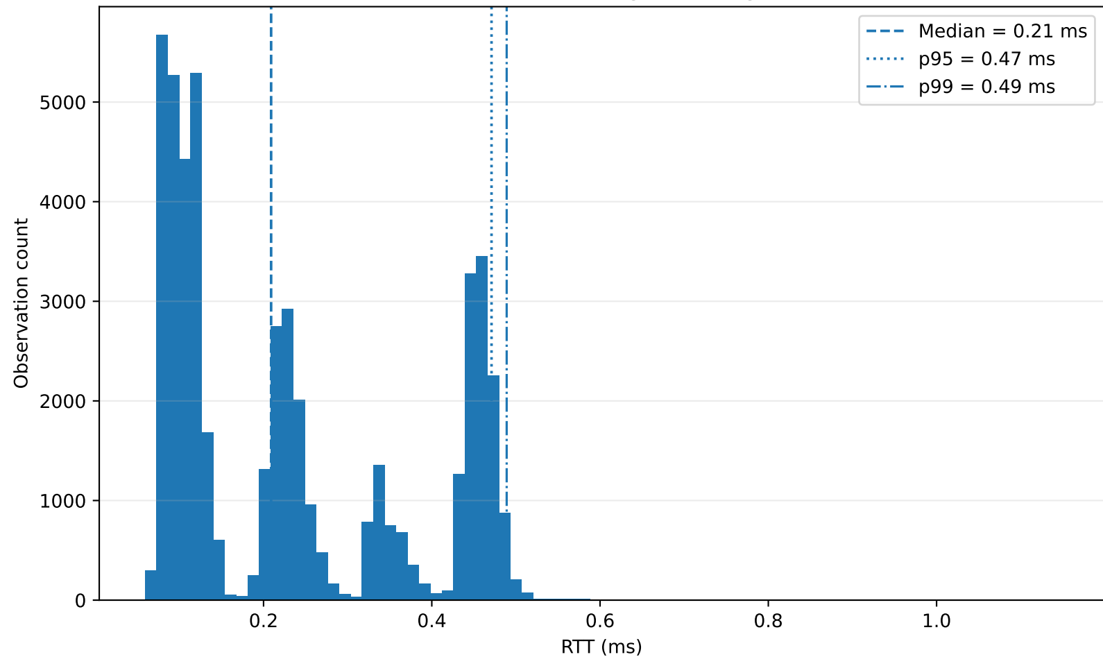
RTT Distribution: Virginia → Virginia
