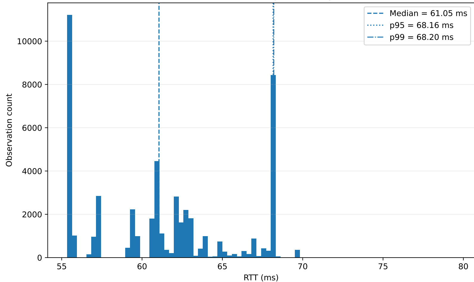
RTT Distribution: Virginia → Oregon
