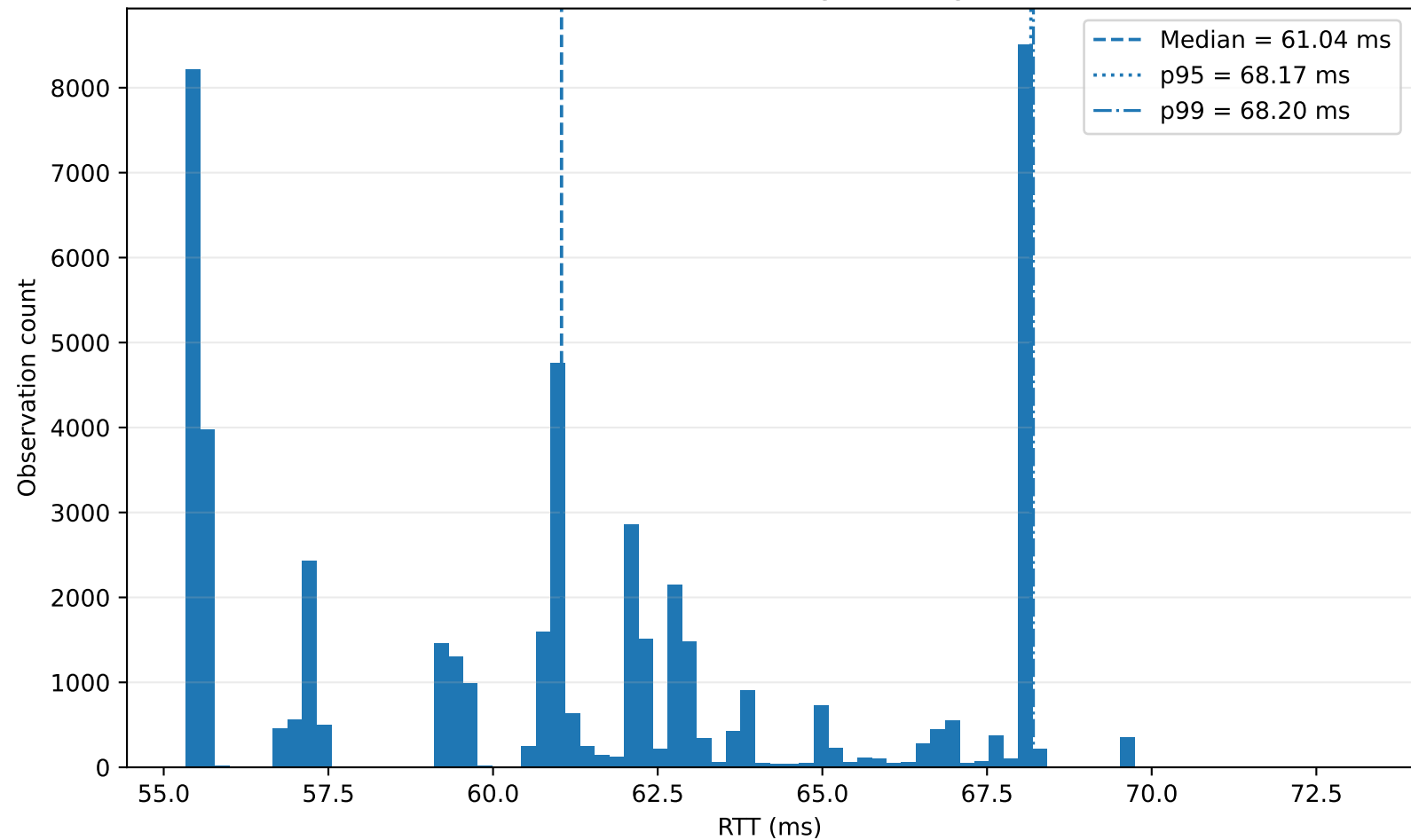
RTT Distribution: Oregon → Virginia
