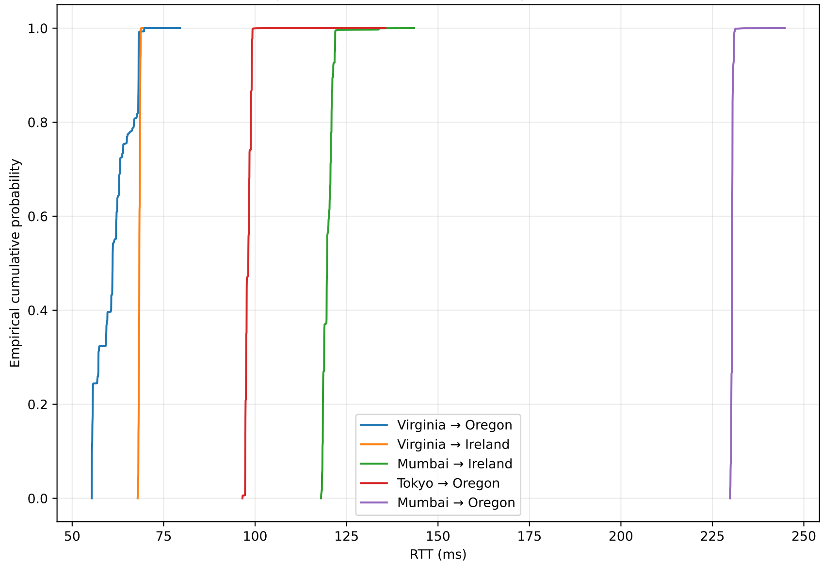
Empirical CDF of Selected Inter-Region RTT Pairs
