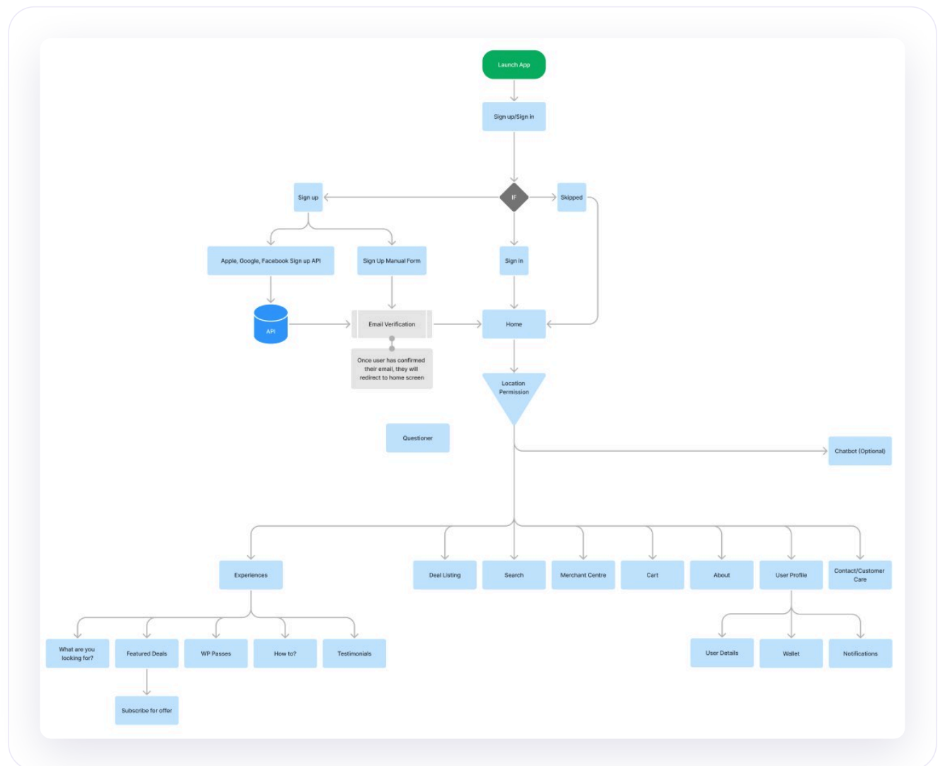
App flow, V1 – sign-up branches on the left, the home-screen sitemap below. "Questioner" and "Chatbot" were parked as optional for a later phase.
