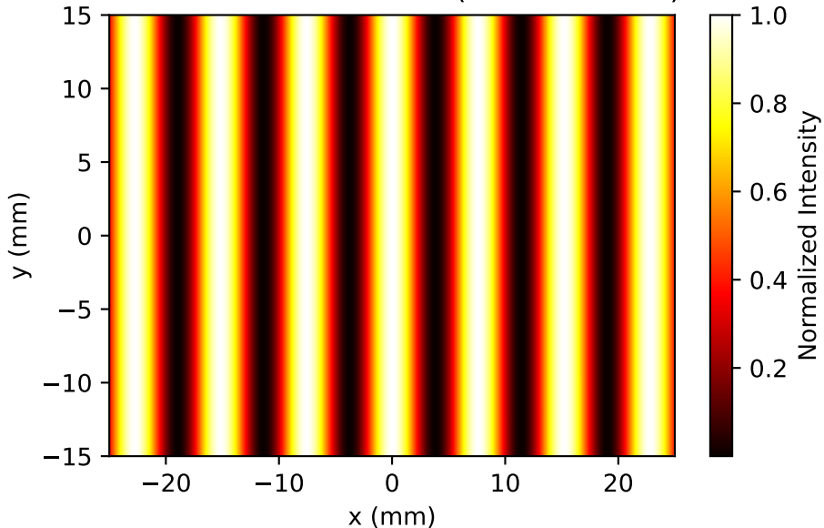
2D Interference Pattern ( d = 0.125 mm)
