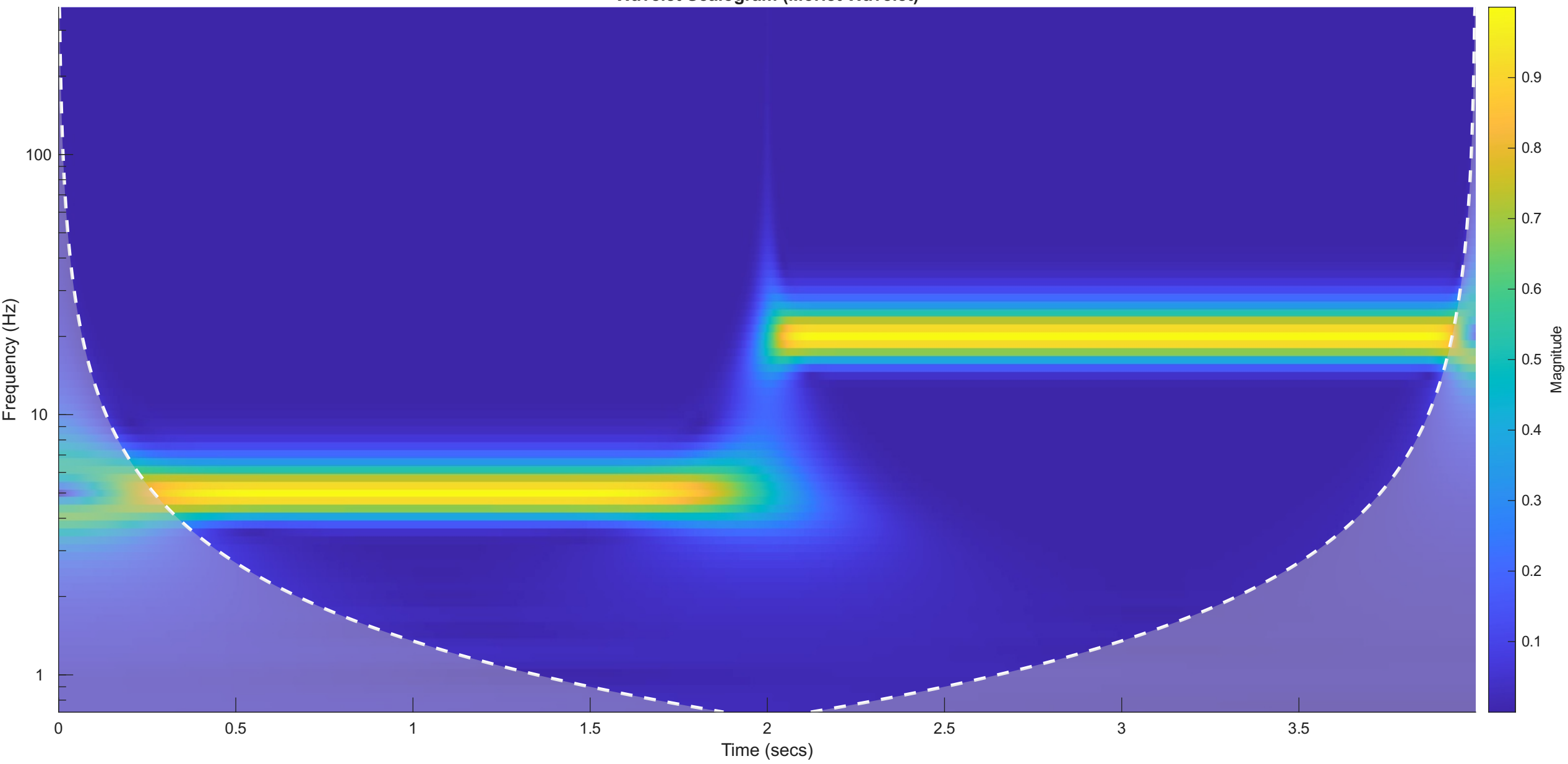
Wavelet Scalogram (Morlet Wavelet)
