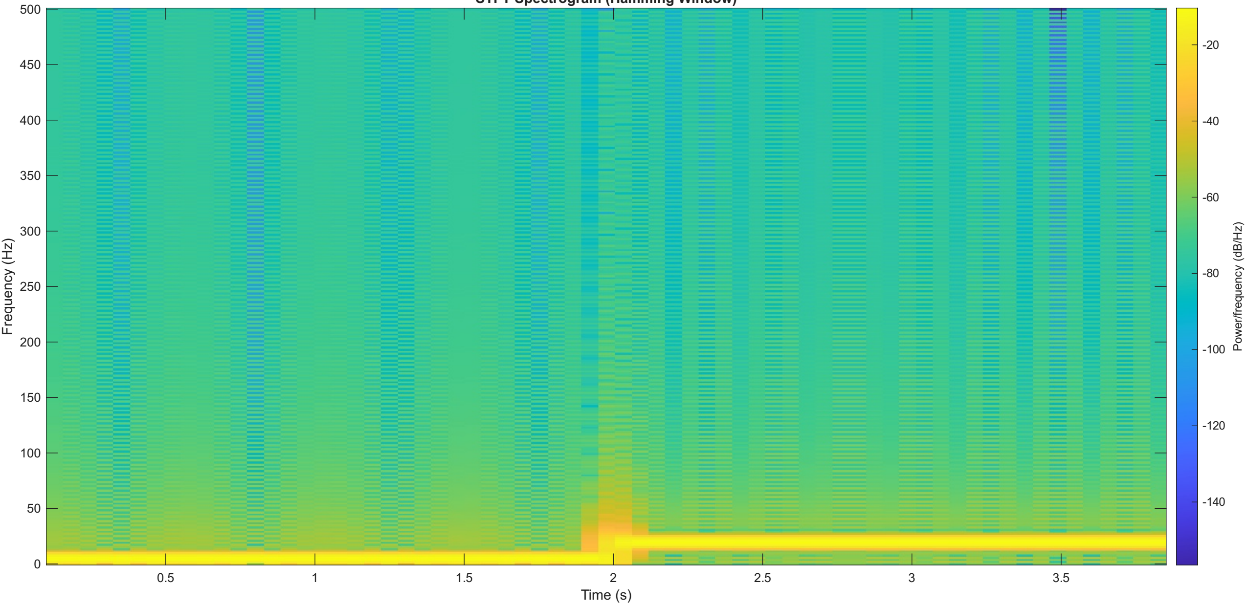
STFT Spectrogram (Hamming Window)
