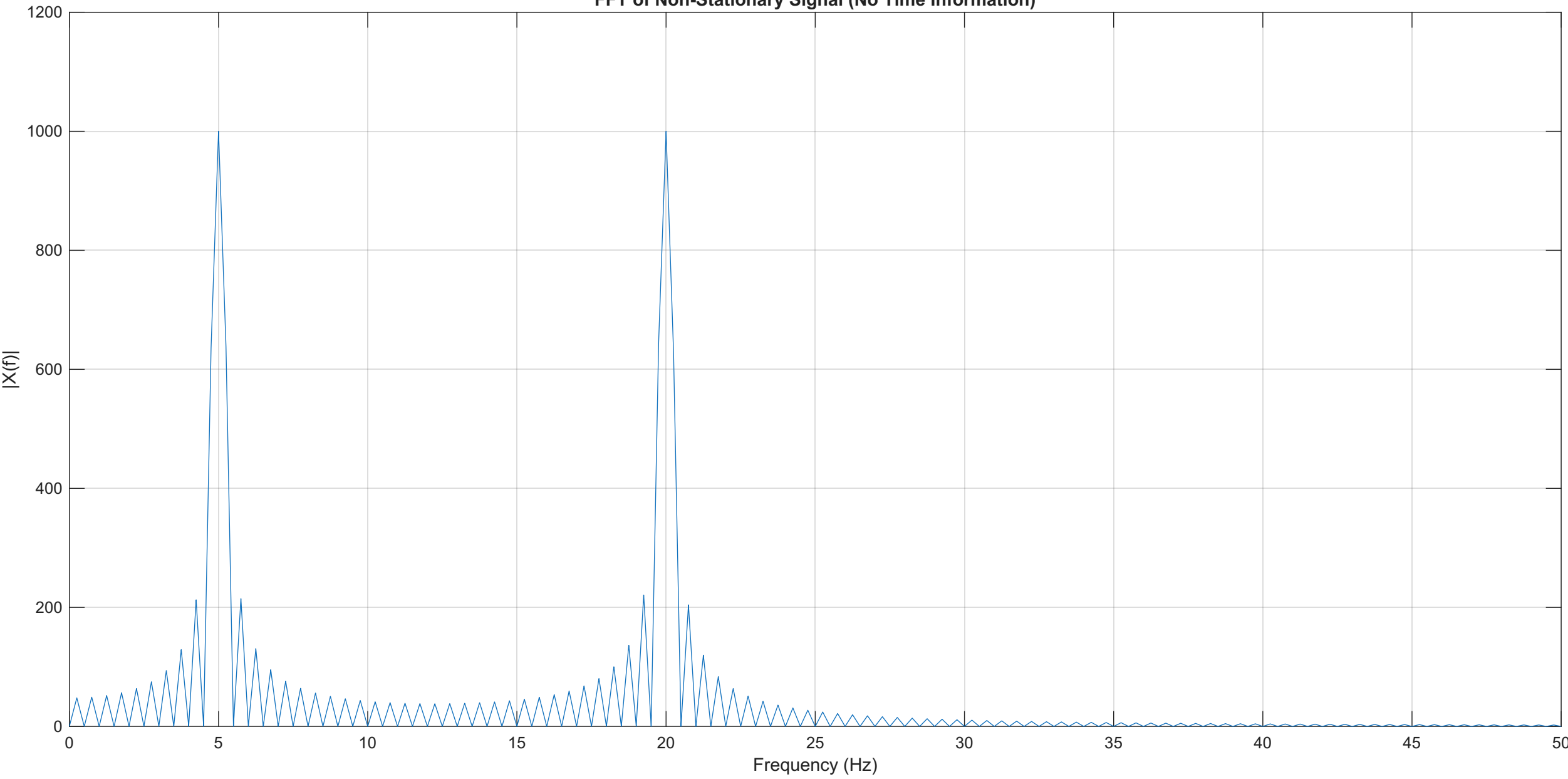
FFT of Non-Stationary Signal (No Time Information)
