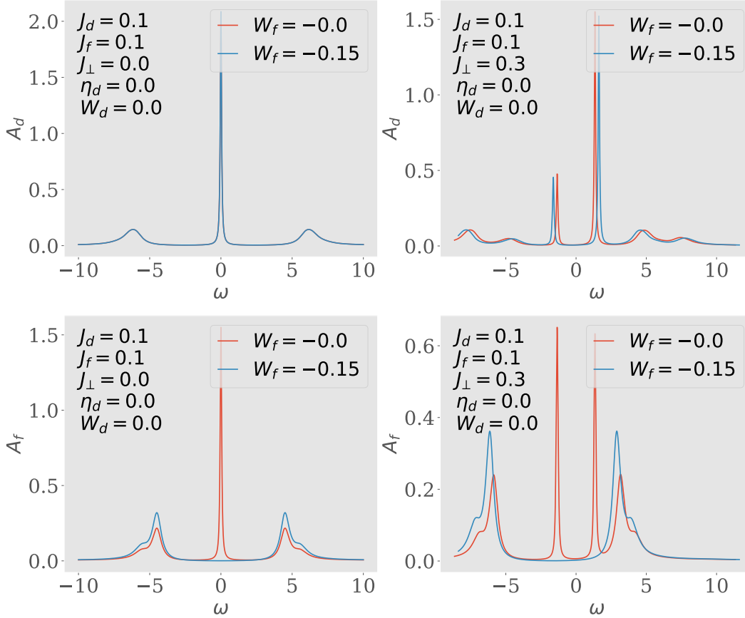
FIG. 10. Spectral functions A_d (top) and A_f (bottom) of the lattice model, for excitations in the d - and f -layers respectively. Both show a central Kondo resonance for J_{\perp} = 0 which splits into two bands upon adding a non-zero J_{\perp} . Increasing |W_f| to large values gaps out the local Fermi liquid excitations of A_f .
