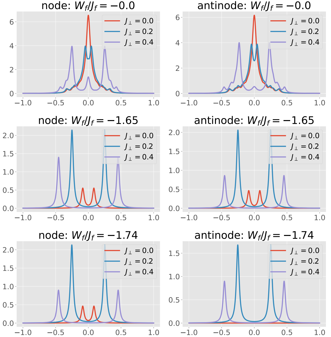
FIG. 12. Spectral functions of the nodal (left) and antinodal (right) k -space point in the f -layer. |W_f| increases from the top panel to the bottom panel, while J_\perp increases within each panel. For small |W_f| , the effect of J_\perp is to create a hybridisation gap in the central resonance of both layers. For large |W_f| , the f -layer is a Mott insulator, and introducing J_\perp then leads to weak metallic processes due to virtual tunneling into the d -layer. These processes again acquire a hybridisation gap at large J_\perp .
