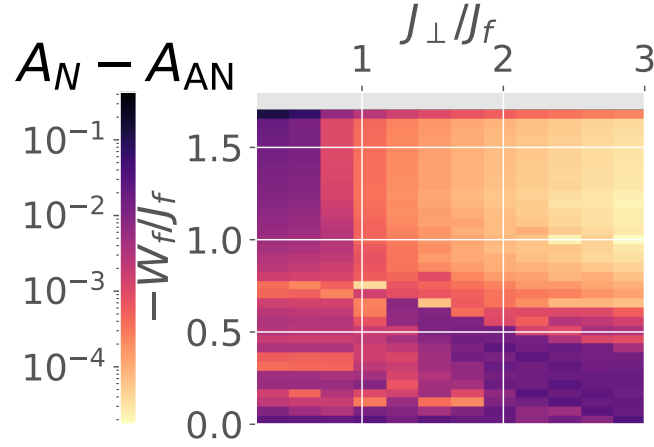
FIG. 13. Anisotropy in the \omega = 0 values between the nodal and antinodal spectral functions for the lattice model. For small |W_f| , we can see an increase in momentum-space differentiation as J_\perp is increased. For large |W_f| , it is instead restricted to small J_\perp . At larger values of |W_f| , the differentiation disappears (gray patch) because both the node and the antinode gap out.
