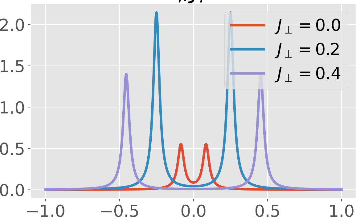
node: W_f/J_f = -1.65
