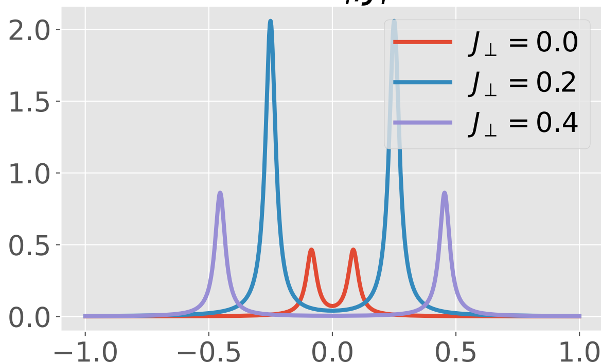
antinode: W_f/J_f = -1.65
