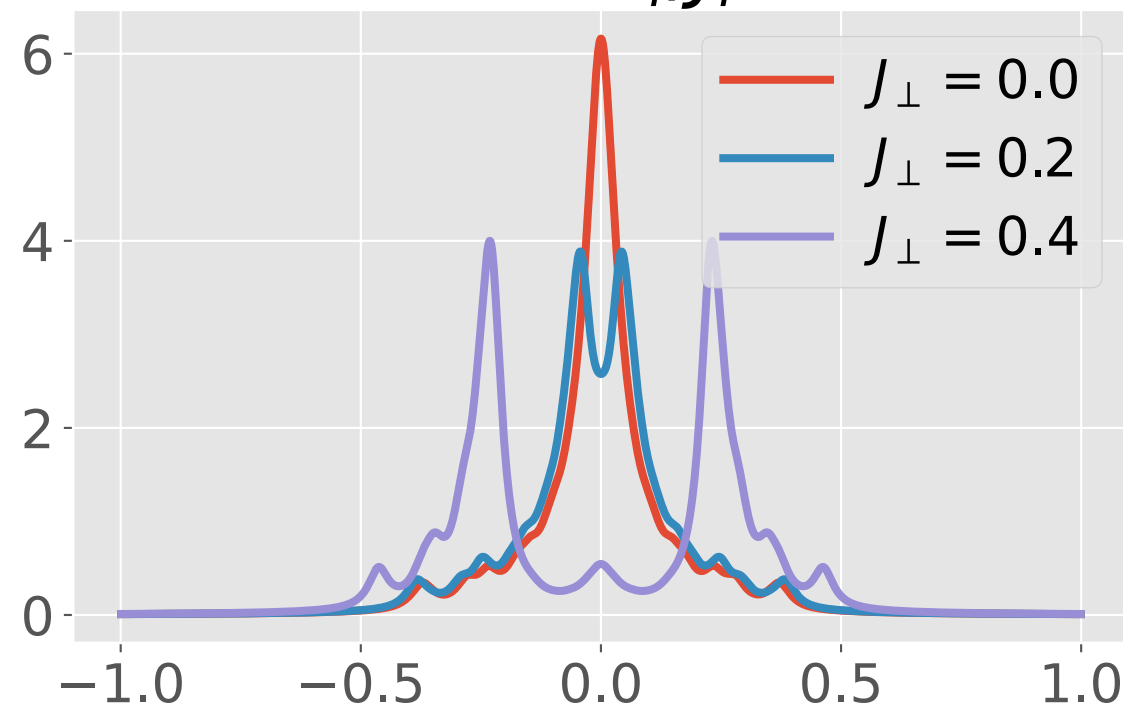
antinode: W_f/J_f = -0.0
