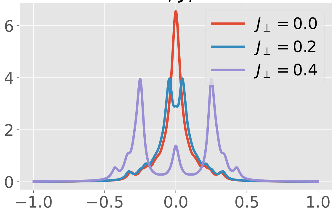
node: W_f/J_f = -0.0
