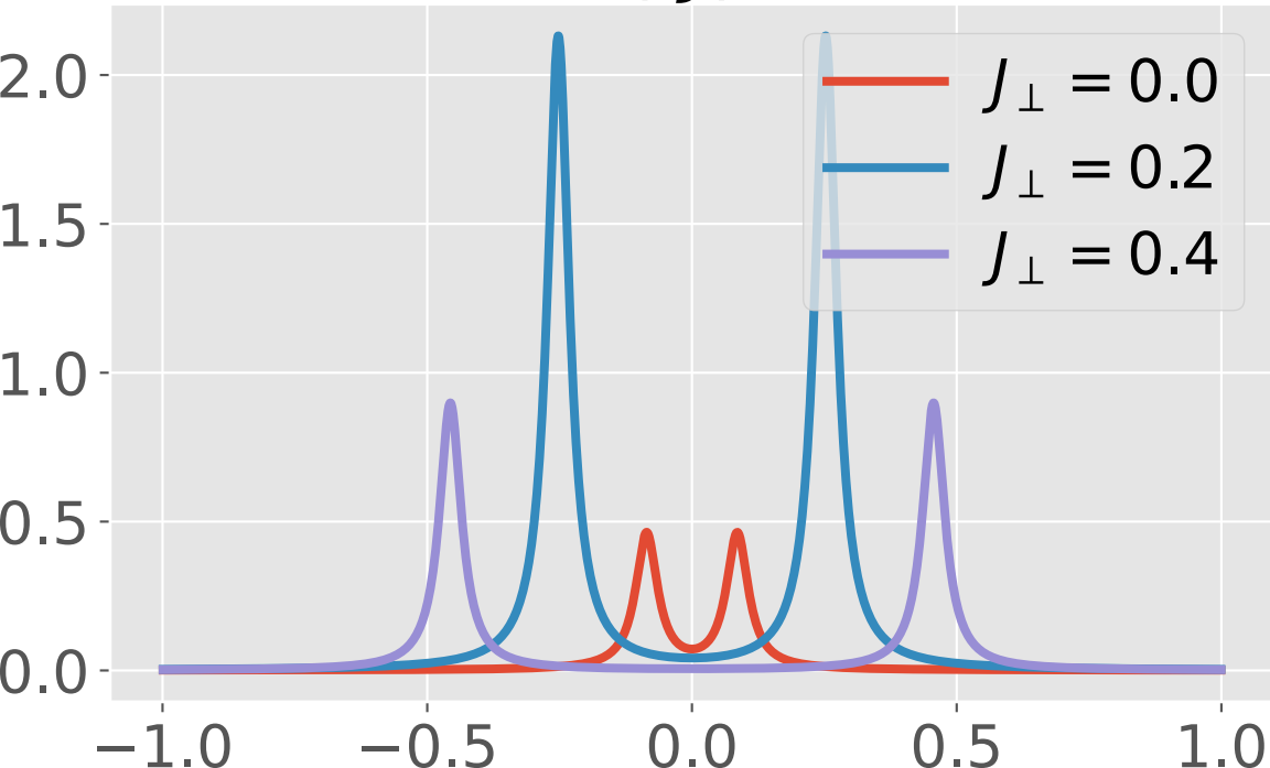
node: W_f/J_f = -1.74
