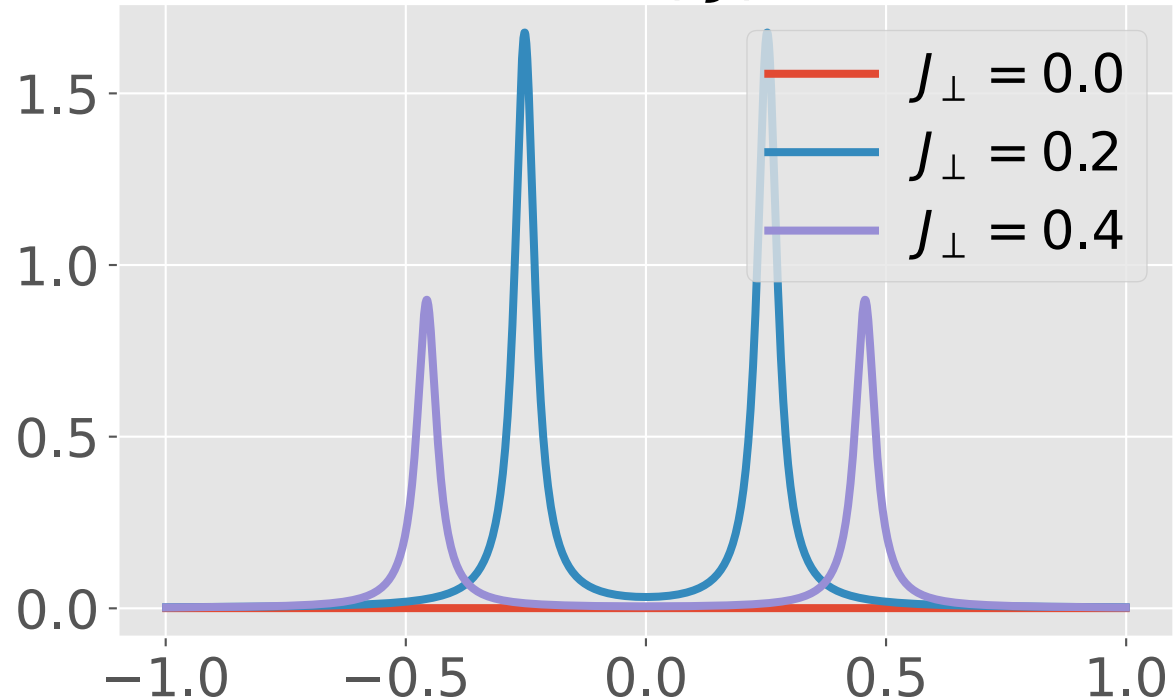
antinode: W_f/J_f = -1.74
