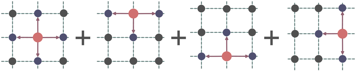
FIG. 1. Depiction of the tiling procedure. Note that each site of the auxiliary model gets mapped to some other site during any given translation operation. This preserves the total number of sites to N .
