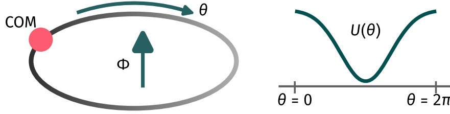
Figure 1.8: The full problem reduces to that of a particle on a circle, in the presence of potential with period 2\pi , and a flux \Phi .
