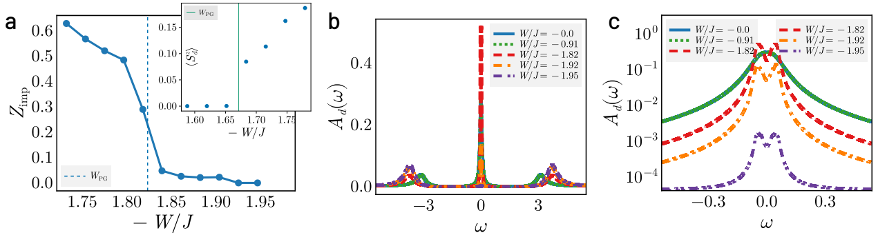
Figure 5.9: (a) Suppression of quasiparticle residue ( Z_{\text{imp}} ) as the impurity model is tuned towards the Mott transition. An initial drastic fall in Z_{\text{imp}} is observed for W/J \lesssim (W/J)_{\text{PG}} from 0.3 to around 0.05, signalling the destruction of the FL with unravelling of Kondo screening. A steady decrease in Z_{\text{imp}} is observed in passage through the PG, and is vanishingly small close to the Mott transition due to a divergent self-energy. Inset shows the growth of unscreened impurity magnetic moment in the pseudogap phase, signalling the breakdown of Kondo screening. (b) Impurity Spectral function in the FL and PG phases. The evolution of the central peak from Kondo resonance to pseudogap is accompanied by dynamical spectral weight transfer to the Hubbard side bands at finite frequencies \omega \simeq \pm 3 (in units of the bandwidth). (c) Zoom-in of the central (Kondo) resonance of the impurity spectral function. While undisturbed in the Fermi liquid phase, it splits into a pseudogap in the PG phase, with its height diminishing rapidly as the Mott transition is approached.
