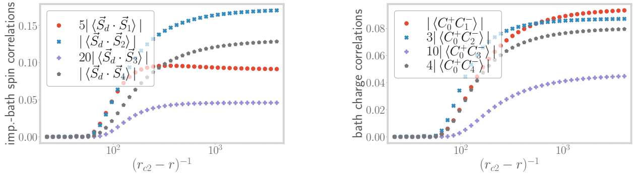
Figure 3.11: Left: Variation of the spin-spin correlations between the impurity and bath sites 1 through 4, close to r_{c2} . They show an increase, revealing the distribution of entanglement into the bath. Right: Variation of pairing correlations within the bath. These correlations show an increase, because of the weakening of the Kondo singlet.
