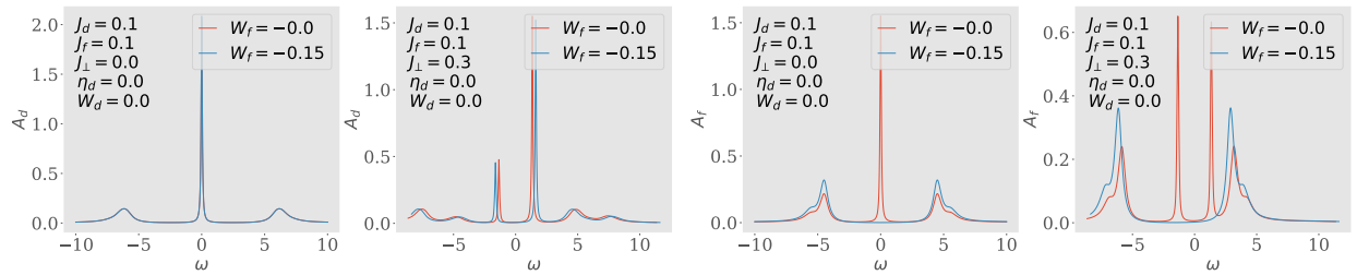
Figure 6.4: Spectral functions A_d and A_f of the auxiliary model, for excitations in the d - and f -layers respectively. Both show a central Kondo resonance for J_\perp = 0 which splits into two bands upon adding a non-zero J_\perp . Increasing |W_f| to large values gaps out the local Fermi liquid excitations of A_f .
