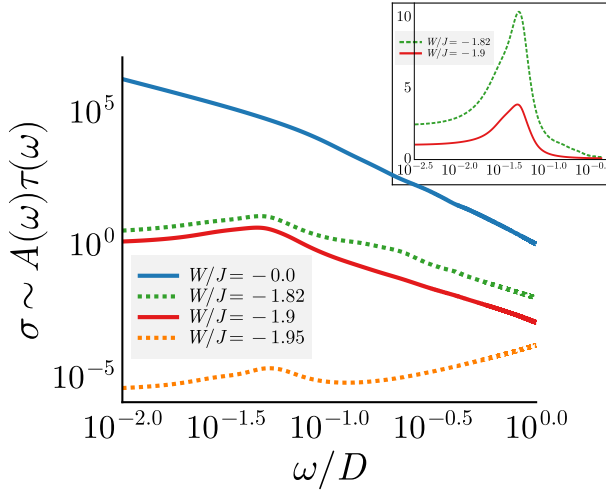
Figure 5.12: Optical conductivity \sigma(\omega) for excitations of the impurity model, approximated through the product of the carrier density (taken from the density of states A(\omega) ) and the lifetime \tau(\omega) (obtained from the inverse scattering rate -1/\Sigma''(\omega) , where \Sigma'' is the imaginary part of the self-energy). The Fermi liquid (blue) shows a sharp Drude peak at \omega = 0 due to the presence of long-lived quasiparticles. The PG (green, red, orange) shows a shifted Drude peak at a non-zero frequency which is reminiscent of the mid-infrared (MIR) peak seen experimentally in the cuprates [512–514]. Inset shows the robustness of the position of the MIR peak through the PG, indicating it as a universal feature of the Mott metal.
