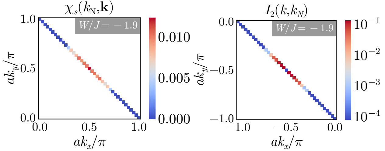
Figure 5.5: Left: Spin correlations \chi_s for the tiled model, between the nodal point k_N = (-\pi/2, -\pi/2) and an arbitrary k -point on the Fermi surface. In the PG, the spin-correlations near the antinode vanish, indicating that they have been removed from the metallic excitations, while the correlations near the nodal point become enhanced because of the increasingly correlated nature of the metal. Right: Mutual information I_2 between an arbitrary k -state and the nodal point. The nodal points remain strongly entangled with each other all the way through the PG.
