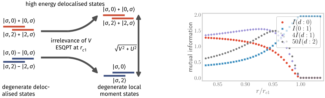
Figure 3.9: Left: Evolution of the excited states mentioned in Eqs. (6.1) as r is tuned through r_{c1} . The high-energy states (red) retain their impurity-bath coupling, while their low-energy counterparts (blue) become disentangled and form a degenerate set of local moment states. The high-energy states allow delocalisation into the bath and lead to the broad Hubbard sidebands. Right: Variation of mutual information (MI) between various parties, across the ESQPT at r_{c1} . The MI (red) between the impurity and the zeroth site vanishes at r_{c1} , showing the localisation of the impurity. The same between the bath zeroth site and the next site becomes maximum at r_{c1} . The MI between the impurity and the other sites (purple and gray) of the bath show an initial rise near r_{c1} , indicating that entanglement is becoming long-ranged near the ESQPT.
