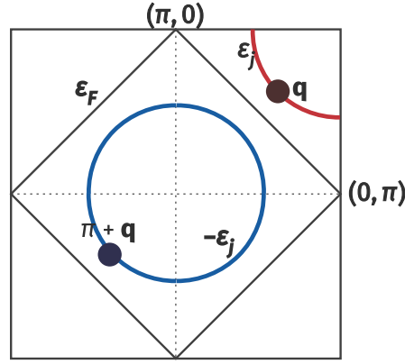
Figure 5.2: Particle and hole states.
