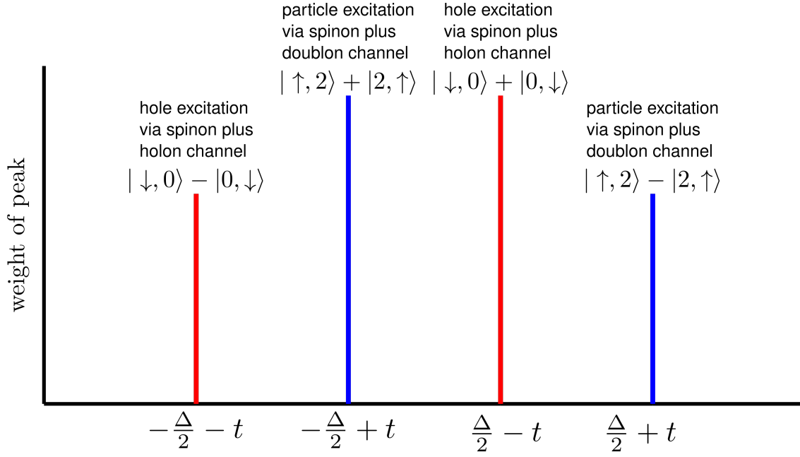
Figure 9.1: Position, weight and nature of each of the peaks in the Hubbard dimer site local spectral function
