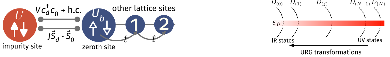
Figure 3.1: Left: Schematic 1D representation of the extended SIAM Hamiltonian. The red sphere is the impurity site with on-site Hubbard term U . It is connected via two couplings V and J to the bath zeroth site (large blue sphere) that has its own on-site Hubbard term U_b . The small blue spheres make up the rest of the bath, connected through the single-particle hopping t . Right: High energy - low energy scheme defined and used in the URG method. The states away from the Fermi surface form the UV subspace and are decoupled first, leading to a Hamiltonian which is more block-diagonal and comprised of only the IR states near the Fermi surface.
