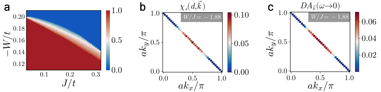
Figure 5.4: (a) Phase diagram of impurity model at strong coupling in U in terms of competing dimensionless Kondo ( J/t ) and bath correlation ( W/t ) couplings. Colourbar represents the fraction of states on the Fermi surface replaced by zeros of the Greens function (Luttinger surface). A pseudogap phase (shaded region) is observed between the local Fermi liquid (red region) and local moment (blue region) phases. (b) k -space-resolved spin-spin correlation \chi_s(d, \mathbf{k}) = \langle \mathbf{S}_d \cdot \mathbf{S}_k \rangle in the pseudogap phase of the impurity model. Antinodal regions are observed to decouple from Kondo screening of the impurity. (c) Upon tiling, this leads to a k -space-resolved antinodal gap in the electronic density of states of the lattice model, corresponding to Luttinger surfaces of zeros.
