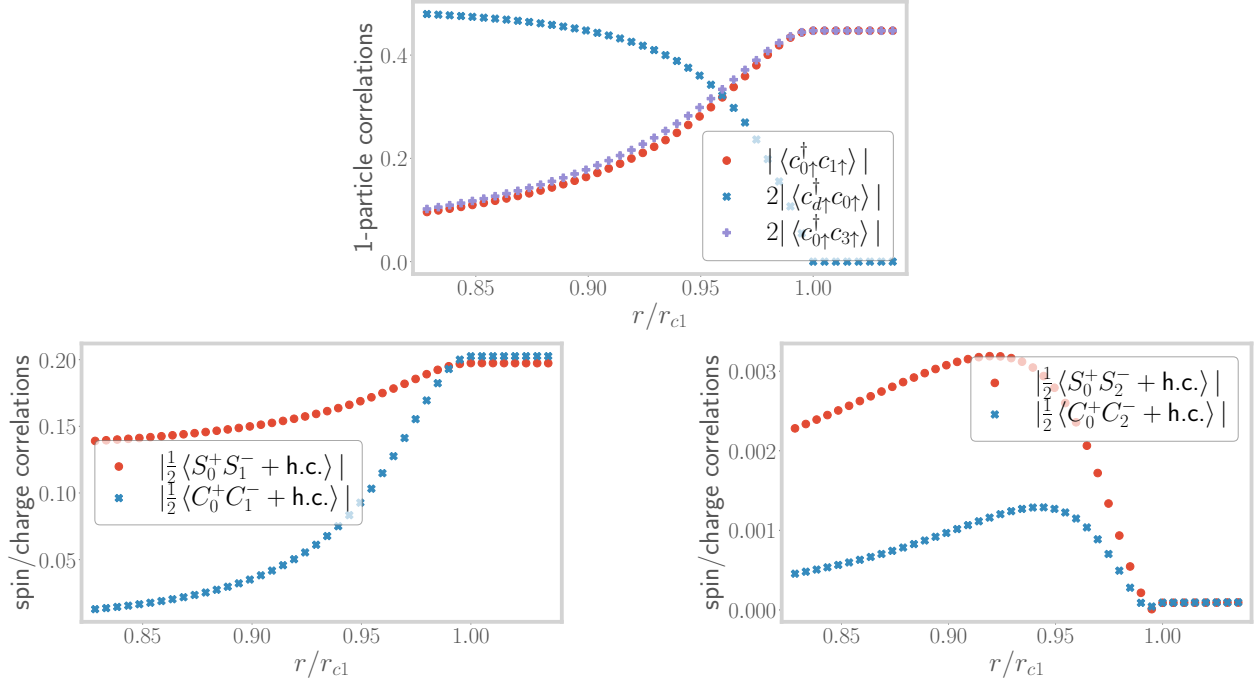
Figure 3.10: Top: Variation of the one particle correlations in the state |1, \sigma, -\rangle between impurity and bath zeroth site (blue), as well as within the bath (red and violet). The former vanishes, depicting the excited state localisation transition at r_{c1} . Left: Variation of the spin-flip (red) and charge isospin-flip (blue) correlations between impurity and bath, close to r_{c1} . They both increase, indicating that the impurity is now less strongly coupled with the bath. Right: Variation of the spin-flip (red) and charge isospin-flip (blue) correlations between the zeroth and second sites of the bath, close to r_{c1} . Both show an initial increase, leading to the propagation of relatively long-range correlations into the bath.
