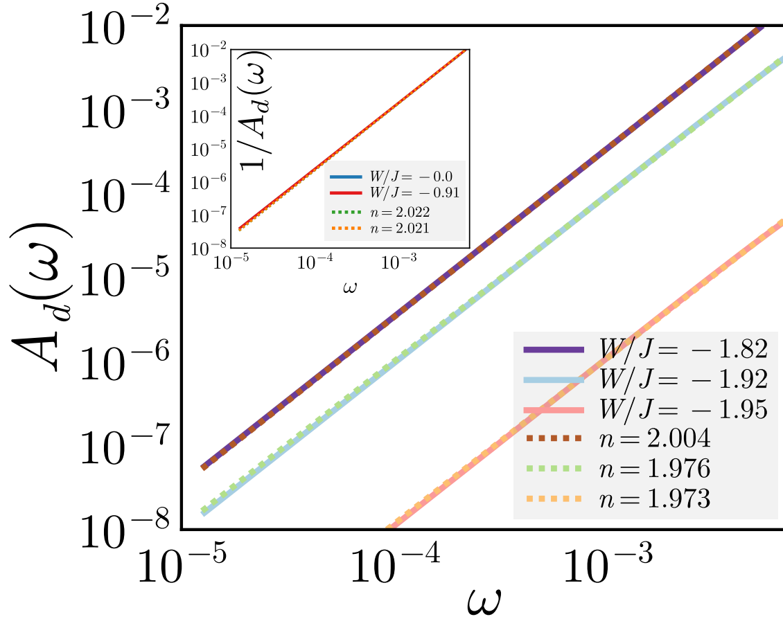
Figure 5.11: Impurity spectral function A_d(\omega) in the local Fermi liquid (inset) and pseudogap (main). The PG spectral function is fit to a power law (with the \omega = 0 contribution subtracted, see Fig. 5.10(c) for the full spectral function). The exponent of the power law comes out to be n \approx 2 throughout the PG. The local FL spectral function (inset) is fit to a lorentzian (by fitting the inverse to a power law).
