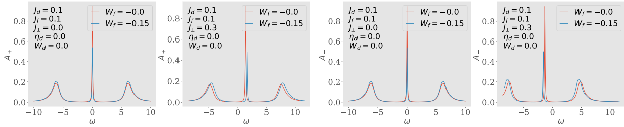
Figure 1.8: Spectral functions of the tiled model, for excitations in the bonding (two on the left) and antibonding (two on the right) basis, defined by the Greens function G_{k,\pm} = G(k_d \pm k_f; \omega) . There is no hybridisation for J_{\perp} = 0 (first and third plots), and the only effect of W_f is to shrink the height of the central resonance. Introducing a non-zero J_{\perp} splits the central resonance into an upper band (second from left) and a lower band (first from right). This leads to a Kondo insulator, where \omega = 0 resides inside the hybridisation gap.
