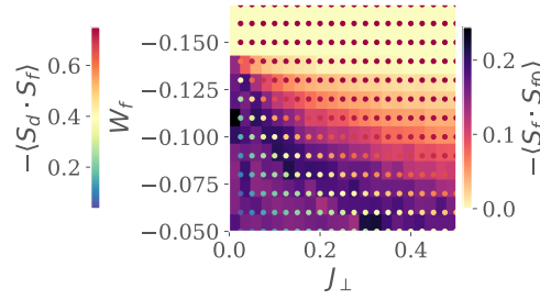
Figure 1.7: Left: Real-space spin correlations for the auxiliary model. Background colour (right colourbar) represents that between the f -impurity and its nearest-neighbour sites, while the marker colour (left colourbar) represents that between the f -impurity and the d -impurity. While the former shrinks as J_{\perp} or |W_f| is increased, the latter grows. This marks a transfer of entanglement from intra-plane channel into inter-plane channel. Right:
