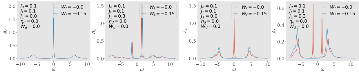
Figure 1.9: Spectral functions A_d and A_f of the auxiliary model, for excitations in the d - and f -layers respectively. Both show a central Kondo resonance for J_{\perp} = 0 which splits into two bands upon adding a non-zero J_{\perp} . Increasing |W_f| to large values gaps out the local Fermi liquid excitations of A_f .
