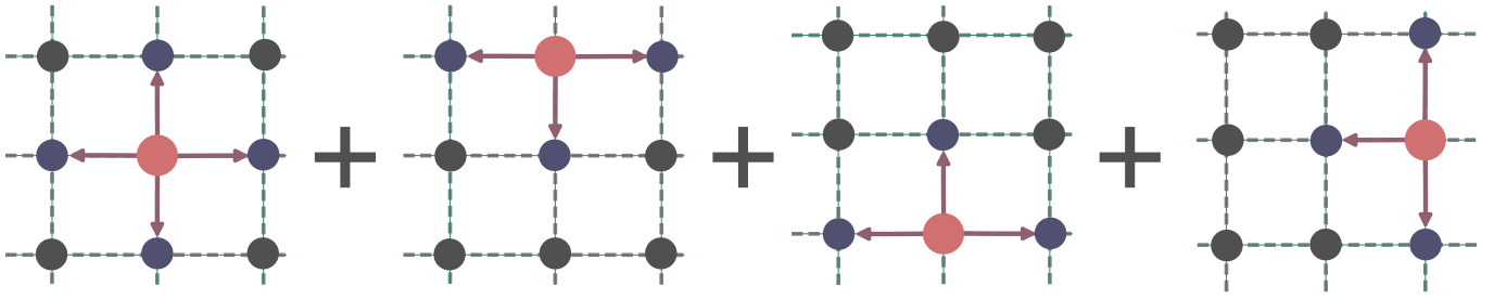
FIG. 2. Depiction of the tiling procedure. Note that each site of the auxiliary model gets mapped to some other site during any given translation operation. This preserves the total number of sites to N .
