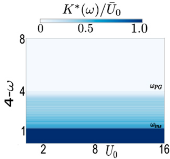
FIG. 1. Transition from a non-Fermi liquid phase (white) to a Mott insulator (dark blue) through a pseudogap (shaded blue), upon lowering the effective quantum fluctuation scale 4 - \omega , via a unitary RG treatment of the Hubbard model on the 2D square lattice at half-filling. Taken from [6].
