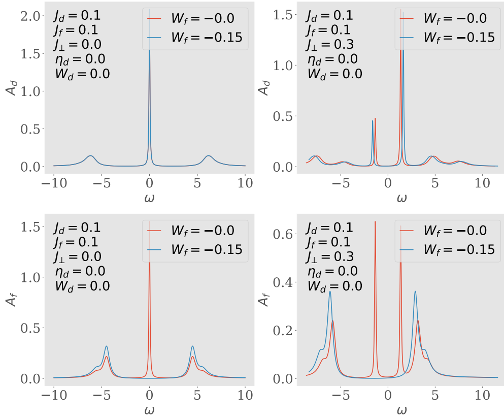
Figure 1.10: Spectral functions A_d (top) and A_f (bottom) of the lattice model, for excitations in the d - and f -layers respectively. Both show a central Kondo resonance for J_\perp = 0 which splits into two bands upon adding a non-zero J_\perp . Increasing |W_f| to large values gaps out the local Fermi liquid excitations of A_f .
