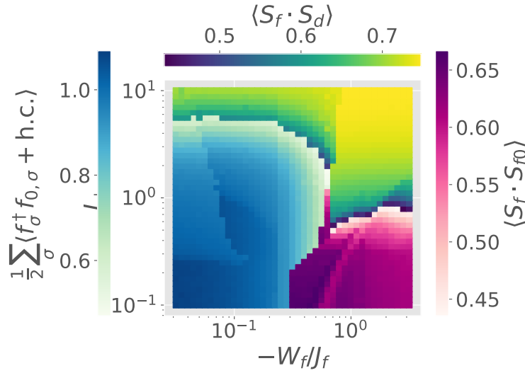
Figure 1.5: Phase diagram of the infinite dimensional impurity model on the Bethe lattice, derived from real-space correlations. The three colors represent three different correlations, defined through the labels. The left half is mostly dominated by the weakly correlated intra-orbital Kondo screened phase where the one-particle correlation between the f -electrons is active (blue color-bar). At small |W_f| , this phase transitions into the inter-orbital screened
