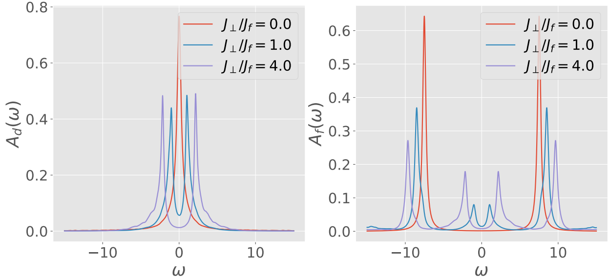
Figure 1.7: Spectral functions of the d - (left) and f -impurity (right), for large |W_f| . The d -impurity shows a splitting of the central resonance because of spin-flip scattering processes with the f -impurity. The f spectral function initially has a Mott gap for small J_\perp . At large J_\perp , scattering processes with the d -layer lead to states at low energies in the form of a pseudogap. Further increasing J_\perp leads to a Kondo insulator.
