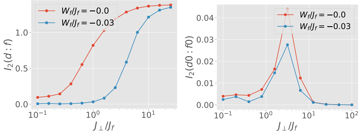
Figure 1.6: Left: Transfer of entanglement during the transition from intra-orbital screened phase to inter-orbital screened phase. For both small (red) and large (blue) |W_f| , the mutual information between the two impurities grows as the inter-orbital screening increases. Right: Close to the transition, we detect an increase in the range of entanglement, through a rise in the value of the mutual information between the zeroth site of the conduction layer and that of the f -layer. This suggests that the transition is marked by a critical point.
