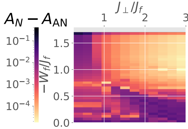
Figure 1.13: Anisotropy in the \omega = 0 values between the nodal and antinodal spectral functions for the lattice model. For small |W_f| , we can see an increase in momentum-space differentiation as J_\perp is increased. For large |W_f| , it is instead restricted to small J_\perp . At larger values of |W_f| , the differentiation disappears (gray patch) because both the node and the antinode gap out.
