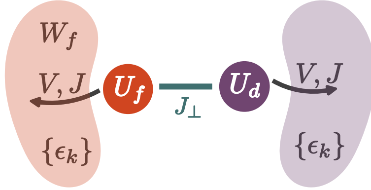
Figure 1.1: The primary workhorse for this chapter is the two impurity auxiliary model. Each impurity hybridises with its own conduction bath. In order to simulate the correlated nature of the f -layer of a lattice model, we will tune the bath correlation W_f to strong values. The impurities interact with each other through the spin-exchange coupling J_\perp .
