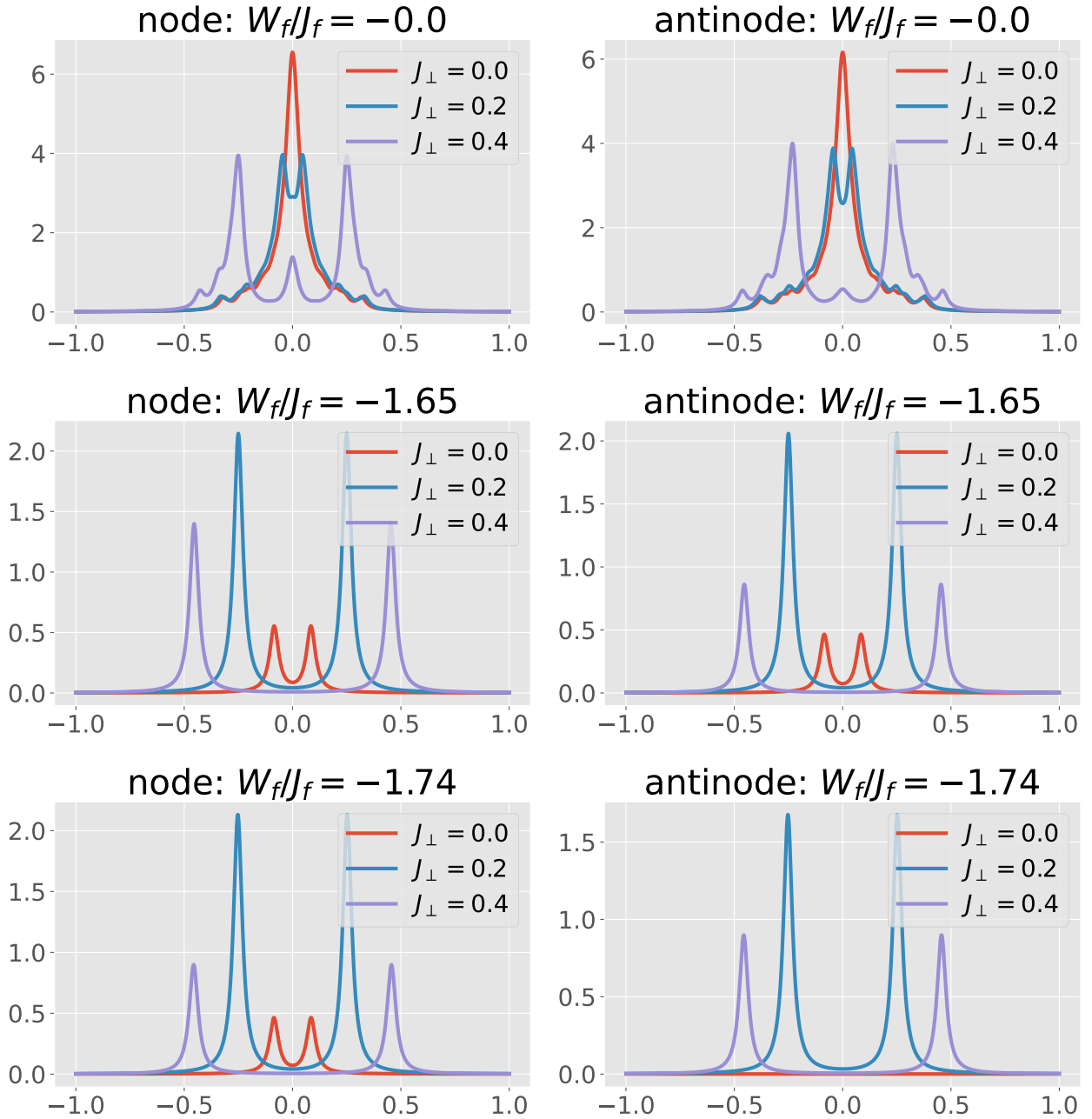
Figure 1.12: Spectral functions of the nodal (left) and antinodal (right) k -space point in the f -layer. |W_f| increases from the top panel to the bottom panel, while J_\perp increases within each panel. For small |W_f| , the effect of J_\perp is to create a hybridisation gap in the central resonance of both layers. For large |W_f| , the f -layer is a Mott insulator, and introducing J_\perp then leads to weak metallic processes due to virtual tunneling into the d -layer. These processes again acquire a hybridisation gap at large J_\perp .
