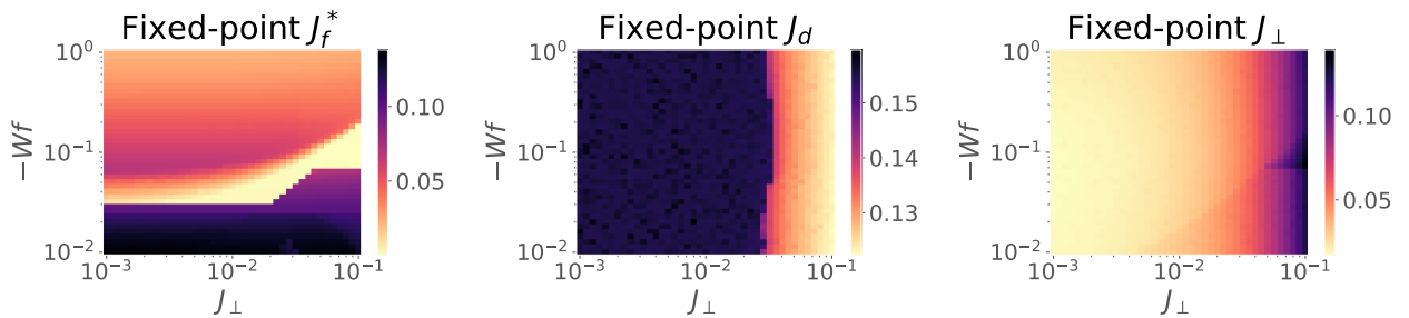
Figure 1.3: Fixed-point values for the direct Kondo couplings J_\alpha and J_\perp . The f -layer Kondo coupling is highly suppressed by increasing both |W_f| and J_\perp . The conduction layer coupling J_d is mildly suppressed by J_\perp . The inter-layer coupling J_\perp itself grows as its bare value is increased. Going from left to right therefore represents a heavy fermion transition from intra-orbital screening at small J_\perp to inter-orbital Kondo screening at large J_\perp .
