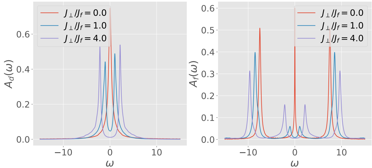
Figure 1.8: Spectral functions of the d - (left) and f -impurity (right), for small |W_f| . The d -impurity again shows a splitting of the central resonance because of spin-flip scattering processes with the f -impurity. In this case, the f -resonance is initially gapless because |W_f| is below its critical value, and it shows behaviour to the d impurity. At large J_\perp , both the spectral functions acquire a hybridisation gap in the spectrum and a Kondo insulator emerges.
