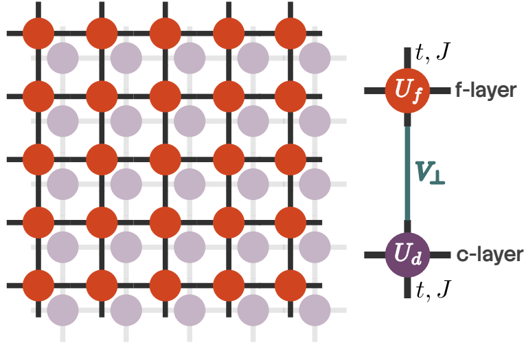
Figure 1.2: Bilayer Hubbard model reconstructed from tiling the two-impurity auxiliary model. The correlated f -layer (orange) hosts a stronger correlation U_f compared to that of the conduction layer (violet) U_d . The two layers are connected by an inter-orbital hybridisation V_\perp .
