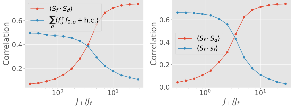
Figure 1.4: Characterisation of the transition for small and large |W_f| in terms of real-space correlation measures. Left: For small |W_f| , the f -layer is weakly correlated and Kondo screening involves both spin and charge degrees of freedom. Accordingly, we track the transition using the charge compensation factor (blue) and the inter-layer spin correlation (red). The charge compensation is suppressed as J_{\perp} is increased and is replaced with the inter-layer correlation, showing the buildup of inter-layer Kondo screening. Right: For large |W_f| , the f -spins are localised and interact with each other through intra-orbital spin correlation \langle S_f \cdot s_f \rangle . As J_{\perp} is increased, these intra-orbital spin correlations are again replaced by inter-orbital spin correlations. In this way, our analysis shows how the inter-orbital correlations replace intra-orbital correlations for both small and large |W_f| .
