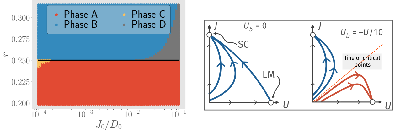
Figure 1.2: Left: Phase diagram of the e -SIAM, in the space of r and J_0/D_0 . U_b is set to -U_0/10 . The various phases are described in the text. Right: Schematic nature of RG flows for U_b = 0 and U_b = -U/10 . Blue curves represent RG flows towards the strong-coupling (SC) fixed point, while red curves represent RG flows towards the local moment (LM) fixed point.
