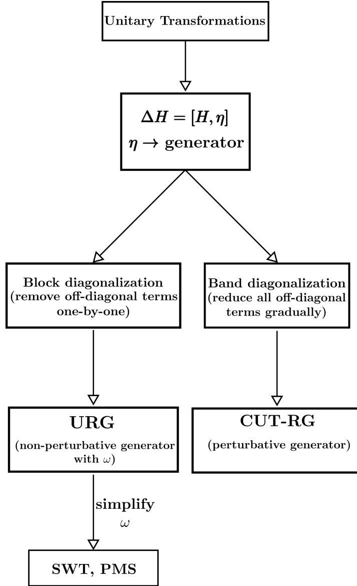
Figure 2.6: Comparison of the various unitary transformations and their relationships to each other.
