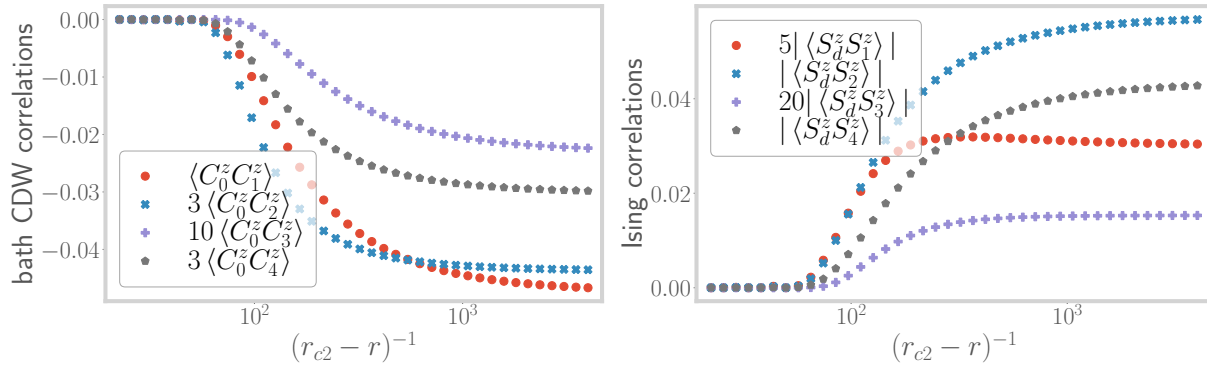
Figure 3.17: Left: Variation of charge isospin Ising correlations between the zeroth site and bath sites further down the chain. Right: Ising correlations between the impurity site and bath sites beyond the zeroth site. Both sets of correlations show an overall increase as r \rightarrow r_{c2} .
