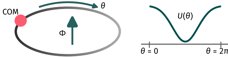
Figure 2.4: The full problem reduces to that of a particle on a circle, in the presence of potential with period 2\pi , and a flux \Phi .
