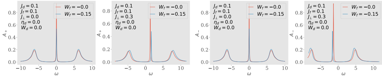
Figure 6.9: Spectral functions of the tiled model, for excitations in the bonding (two on the left) and antibonding (two on the right) basis, defined by the Greens function G_{k,\pm} = G(k_d \pm k_f; \omega) . There is no hybridisation for J_{\perp} = 0 (first and third plots), and the only effect of W_f is to shrink the height of the central resonance. Introducing a non-zero J_{\perp} splits the central resonance into an upper band (second from left) and a lower band (first from right). This leads to a Kondo insulator, where \omega = 0 resides inside the hybridisation gap.
