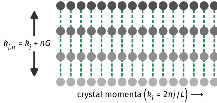
Figure 2.2: The complete set of momentum states in the system. Each row represents a band of states. Each column contains the set of momenta that are connected by a reciprocal lattice vector nG . The states in the lowest band give rise to the crystal momenta. All the momentum states in a column are connected to each other through the potential term (green dotted line). Any two states within a band, on the other hand, are decoupled from each other.
