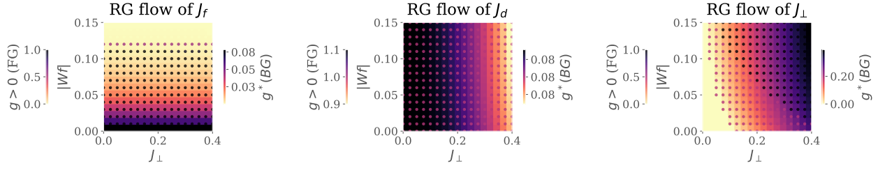
Figure 6.7: RG phase diagrams for various Kondo couplings: f -layer (left), d -layer (middle) and inter-layer (right). For each plot, the background color (quantified by the right colorbar) tracks the fixed point value of the coupling as a function of the inter-layer couplings J_{\perp} and the f -layer bath interaction |W_f| . The marker color complements this by tracking whether the coupling is relevant, intermediate-coupling or irrelevant in the RG sense, by taking the values 1, 1/2 or 0 respectively.
