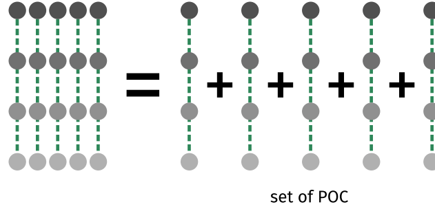
Figure 2.3: Because of the periodicity of the potential, the problem splits into a sum of particle on a circle (POC) problems, each formed by a specific crystal momentum and other momentum states that are related to it by a reciprocal vector.
