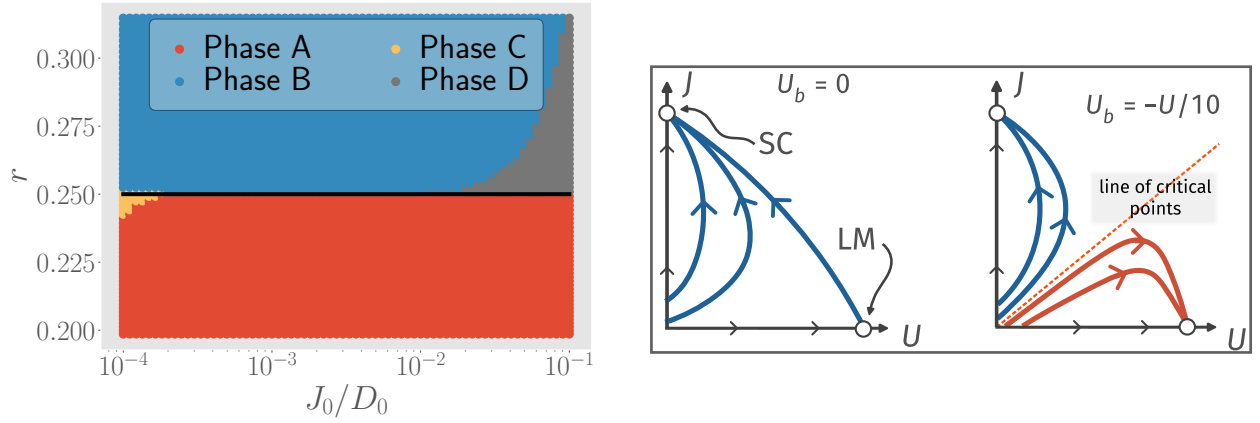
Figure 3.2: Left: Phase diagram of the e -SIAM, in the space of r and J_0/D_0 . U_b is set to -U_0/10 . The various phases are described in the text. Right: Schematic nature of RG flows for U_b = 0 and U_b = -U/10 . Blue curves represent RG flows towards the strong-coupling (SC) fixed point, while red curves represent RG flows towards the local moment (LM) fixed point.
