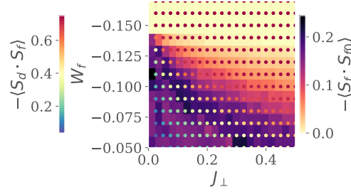
Figure 6.8: Left: Real-space spin correlations for the auxiliary model. Background colour (right colourbar) represents that between the f -impurity and its nearest-neighbour sites, while the marker colour (left colourbar) represents that between the f -impurity and the d -impurity. While the former shrinks as J_{\perp} or |W_f| is increased, the latter grows. This marks a transfer of entanglement from intra-plane channel into inter-plane channel. Right:
