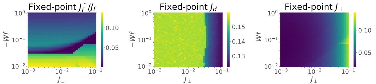
Figure 6.1: Fixed-point values for the direct Kondo couplings J_{\alpha} and J_{\perp} .
