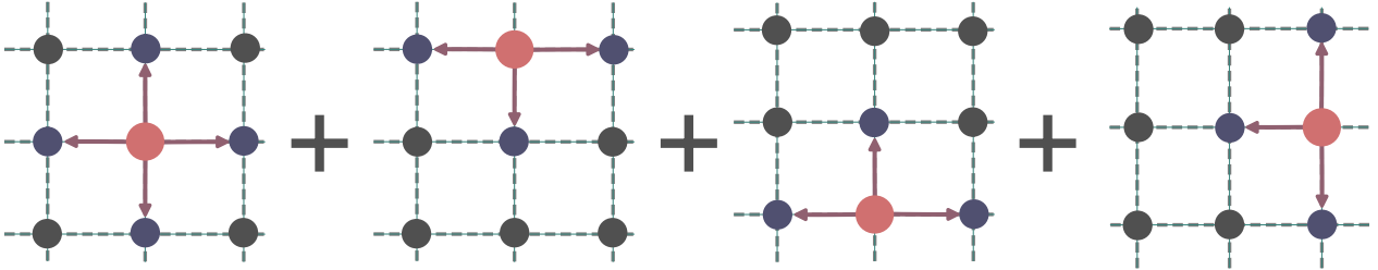
Figure 1.17: Schematic depiction of the "tiling" step in our auxiliary model approach. In order to restore translation invariance and map our impurity model to a lattice model, we apply manybody translation operators on our impurity model Hamiltonian for all lattice sites; this reconstructs the full lattice model, and leads to relations between the auxiliary model couplings and the lattice model couplings.
