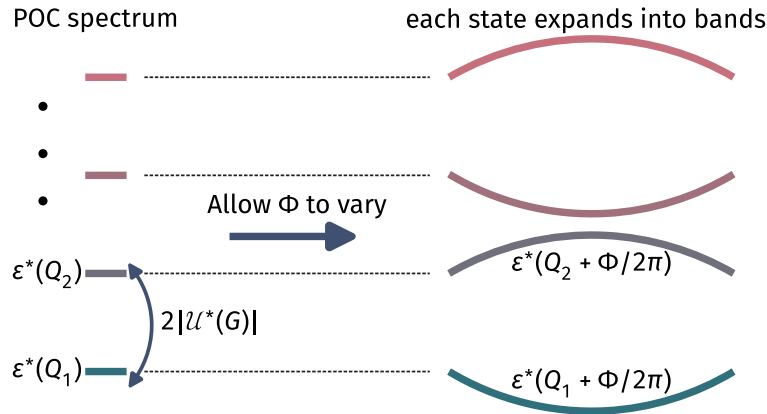
Figure 2.5: Spectral flow transformations on the POC by tuning the flux \Phi generates the full band of delocalised single-particle electronic states whose crystal momenta correspond to \hbar\Phi/a .
