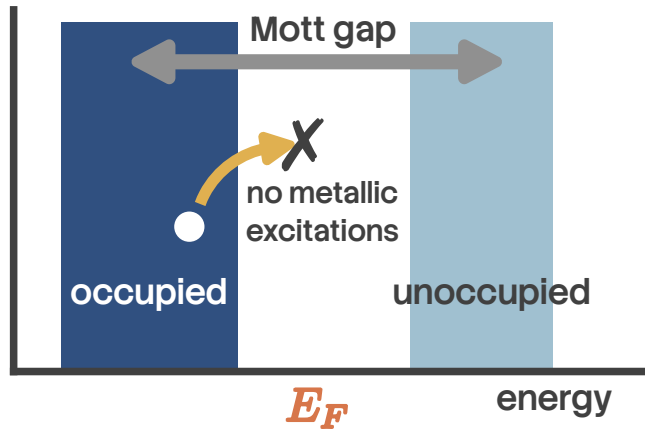
Interactions lead to a Mott Insulator
