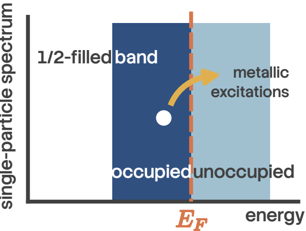
Metal according to band theory
