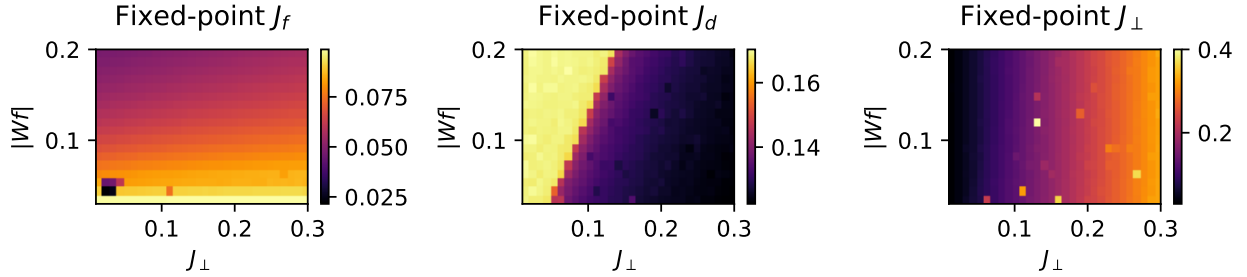
Figure 1.2: Fixed-point values for the direct Kondo couplings J_\alpha and J_\perp for K_\alpha = -10^{-6} .
