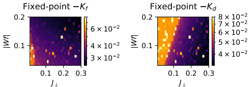
Figure 1.3: Fixed-point values for the indirect Kondo couplings K_\alpha for K_\alpha = -10^{-6} .
