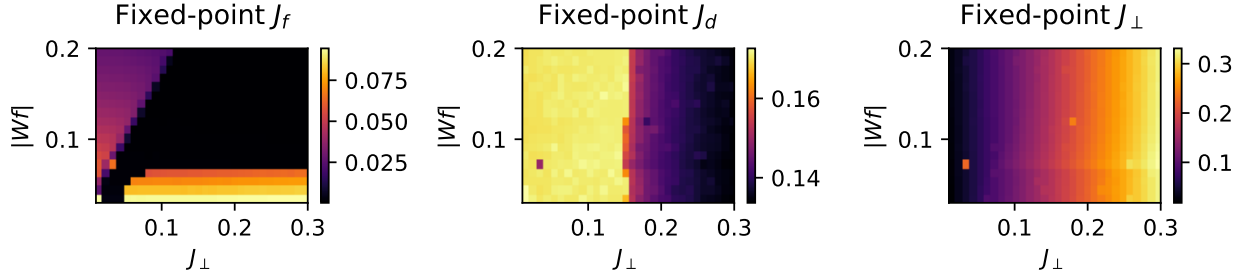
Figure 1.1: Fixed-point values for the direct Kondo couplings J_\alpha and J_\perp for K_\alpha = 0 .
