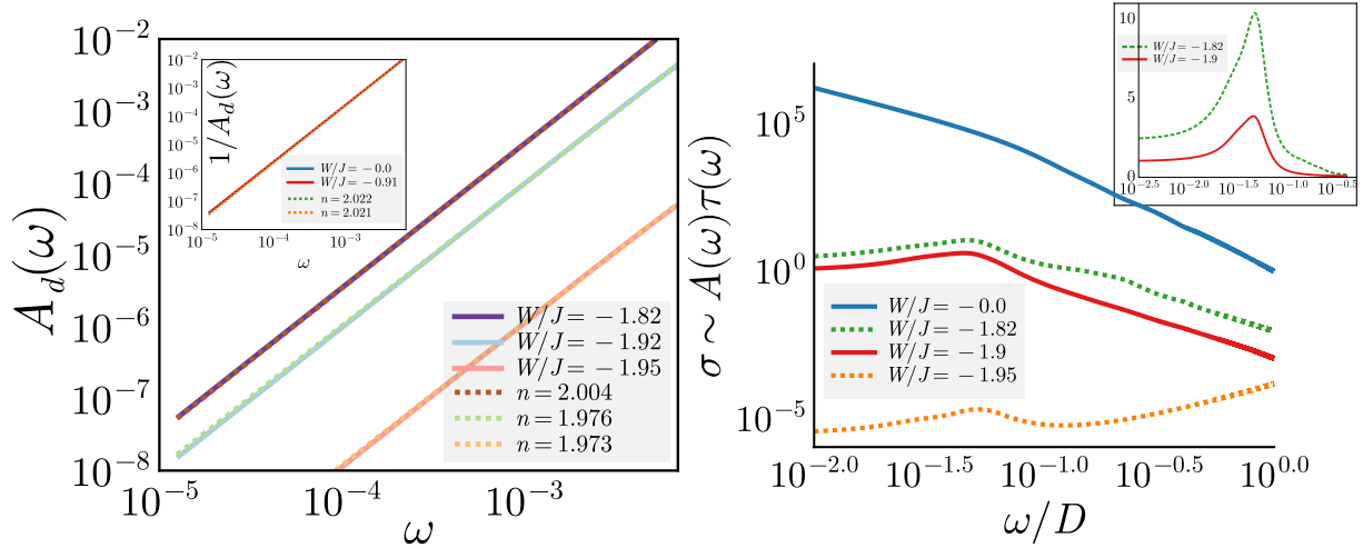
Figure 1.12: Left: Impurity spectral function A_d(\omega) in the local Fermi liquid (inset) and pseudogap (main). The PG spectral function is fit to a power law (with the \omega = 0 contribution subtracted, see Fig. 1.11(c) for the full spectral function). The exponent of the power law comes out to be n \approx 2 throughout the PG. The local FL spectral function (inset) is fit to a lorentzian (by fitting the inverse to a power law). Right: Optical conductivity \sigma(\omega) for excitations of the impurity model, approximated through the product of the carrier density (taken from the density of states A(\omega) ) and the lifetime \tau(\omega) (obtained from the inverse scattering rate -1/\Sigma''(\omega) , where \Sigma'' is the imaginary part of the self-energy). The Fermi liquid (blue) shows a sharp Drude peak at \omega = 0 due to the presence of long-lived quasiparticles. The PG (green, red, orange) shows a shifted Drude peak at a non-zero frequency which is reminiscent of the mid-infrared (MIR) peak seen experimentally in the cuprates [64–66]. Inset shows the robustness of the position of the MIR peak through the PG, indicating it as a universal feature of the Mott metal.
