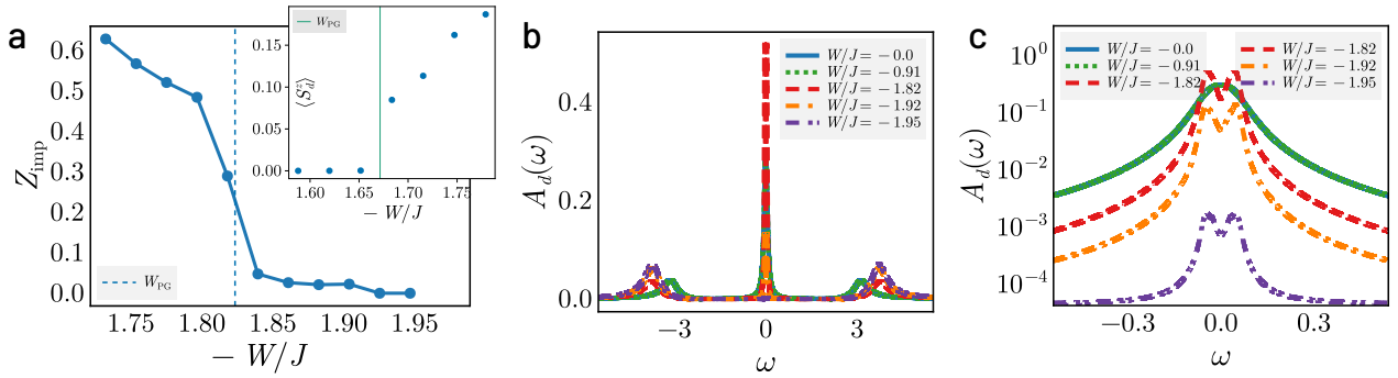
Figure 1.10: (a) Suppression of quasiparticle residue ( Z_{\text{imp}} ) as the impurity model is tuned towards the Mott transition. An initial drastic fall in Z_{\text{imp}} is observed for W/J \lesssim (W/J)_{\text{PG}} from 0.3 to around 0.05, signalling the destruction of the FL with unravelling of Kondo screening. A steady decrease in Z_{\text{imp}} is observed in passage through the PG, and is vanishingly small close to the Mott transition due to a divergent self-energy. Inset shows the growth of unscreened impurity magnetic moment in the pseudogap phase, signalling the breakdown of Kondo screening. (b) Impurity Spectral function in the FL and PG phases. The evolution of the central peak from Kondo resonance to pseudogap is accompanied by dynamical spectral weight transfer to the Hubbard side bands at finite frequencies \omega \simeq \pm 3 (in units of the bandwidth). (c) Zoom-in of the central (Kondo) resonance of the impurity spectral function. While undisturbed in the Fermi liquid phase, it splits into a pseudogap in the PG phase, with its height diminishing rapidly as the Mott transition is approached.
