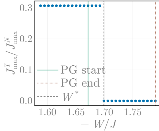
Figure 1.8: Ratio between the maximum values of the fixed point values of the Kondo couplings for scattering processes between and within the regions S^+ and S^- . The vanishing of the fixed point ratio indicates that the pseudogap regime features a singular low-energy effective theory, where the Fermi surface neighbourhood splits into two disconnected regions with no explicit term in the Hamiltonian connecting them directly.
