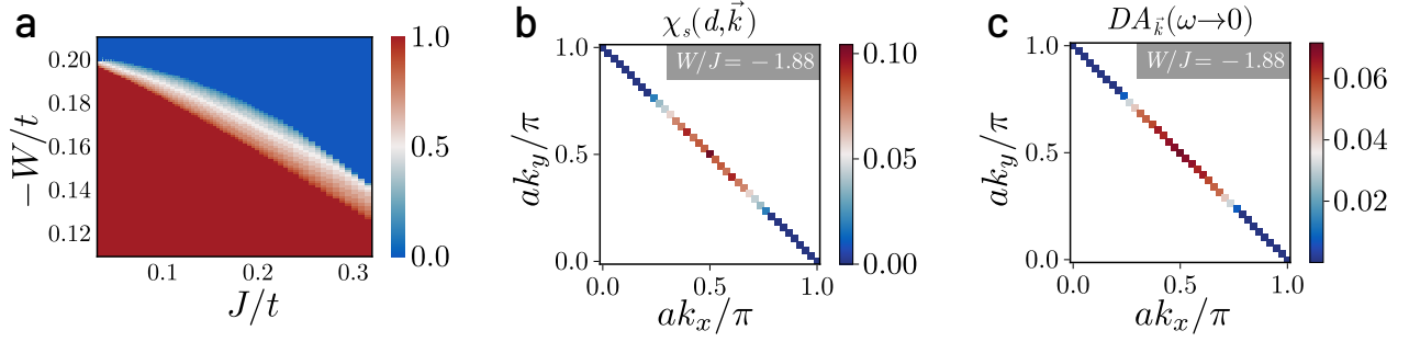
Figure 1.5: (a) Phase diagram of impurity model at strong coupling in U in terms of competing dimensionless Kondo ( J/t ) and bath correlation ( W/t ) couplings. Colourbar represents the fraction of states on the Fermi surface replaced by zeros of the Greens function (Luttinger surface). A pseudogap phase (shaded region) is observed between the local Fermi liquid (red region) and local moment (blue region) phases (b) k -space-resolved spin-spin correlation \chi_s(d, \mathbf{k}) = \langle \mathbf{S}_d \cdot \mathbf{S}_{\mathbf{k}} \rangle in the pseudogap phase of the impurity model. Antinodal regions are observed to decouple from Kondo screening of the impurity. (c) Upon tiling, this leads to a k -space-resolved antinodal gap in the electronic density of states of the lattice model, corresponding to Luttinger surfaces of zeros.
