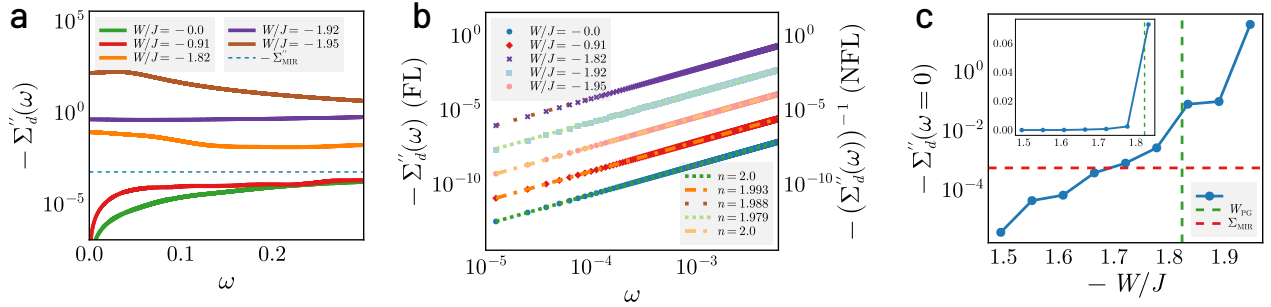
Figure 1.11: (a) Imaginary part of impurity self-energy \Sigma''(\omega) as a function of frequency \omega for Fermi liquid (FL, |W/J| < 1.79 ) and pseudogapped phases (NFL, |W/J| \geq 1.79 ). \Sigma''(\omega) falls to zero as \omega \rightarrow 0 for the FL, while it attains a peak in the pseudogap. All \Sigma''(\omega) for the NFL are observed to lie above the Mott-Ioffe-Regel (MIR) bound (dashed blue line), while those for the FL lie below. (b) Scaling of \Sigma''(\omega) with frequency for Fermi liquid and pseudogapped phases. The FL self-energy fits to \Sigma'' \sim \omega^\alpha with \alpha \approx 2 , vanishing as \omega \rightarrow 0 , while the NFL self-energy grows as \Sigma'' \approx a - \omega^\beta for small \omega , with \beta \approx 2 . Remarkably, the NFL exponent remains mostly unchanged through the entirety of the PG phase. (c) Variation of the zero-frequency imaginary self-energy -\Sigma''(\omega = 0) with \omega in the FL and pseudogap phases (entry into the PG is marked by the vertical dashed line). The inset shows the same but in linear scale, in order to display the dramatic rise (by almost 30 times) on entering the PG.
