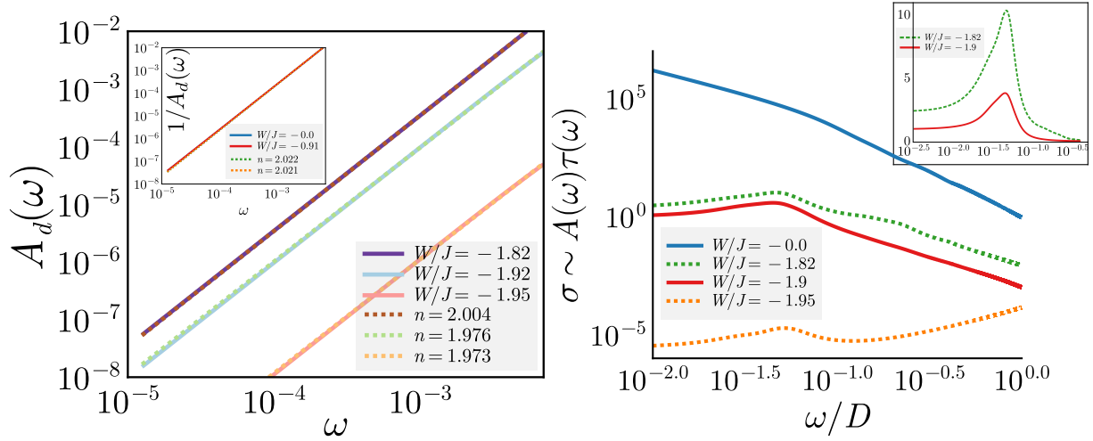
Figure 5.11: Left: Impurity spectral function A_d(\omega) in the local Fermi liquid (inset) and pseudogap (main). The PG spectral function is fit to a power law (with the \omega = 0 contribution subtracted, see Fig. 5.10(c) for the full spectral function). The exponent of the power law comes out to be n \approx 2 throughout the PG. The local FL spectral function (inset) is fit to a lorentzian (by fitting the inverse to a power law). Right: Optical conductivity \sigma(\omega) for excitations of the impurity model, approximated through the product of the carrier density (taken from the density of states A(\omega) ) and the lifetime \tau(\omega) (obtained from the inverse scattering rate -1/\Sigma''(\omega) , where \Sigma'' is the imaginary part of the self-energy). The Fermi liquid (blue) shows a sharp Drude peak at \omega = 0 due to the presence of long-lived quasiparticles. The PG (green, red, orange) shows a shifted Drude peak at a non-zero frequency which is reminiscent of the mid-infrared (MIR) peak seen experimentally in the cuprates [Herr et al.(1987)Herr, Kamarás, Porter, Doss, Tanner, Bonn, Greedan, Stager, and Timusk, Orenstein et al.(1987)Orenstein, Thomas, Rapkine, Bethea, Levine, Cava, Rietman, and Johnson, Uchida et al.(1991)Uchida, Ido, Takagi, Arima, Tokura, and Tajima]. Inset shows the robustness of the position of the MIR peak through the PG, indicating it as a universal feature of the Mott metal.
