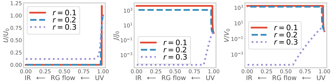
Figure 3.3: Variation of couplings U, V and J along the RG transformations, for three values of the transition-tuning ratio r = -U_b/J_0 . The x-axis represents the distance of the running cutoff from the Fermi surface; the rightmost point is the first RG step (UV) and the leftmost point is the final RG step (IR). The red curves represent the flows for r < r_{c1} , where both V and J are relevant. The blue curves represent the RG flows for r_{c1} < r < r_{c2} , where J is relevant but V is irrelevant. The violet curves represent RG flows for r > r_{c2} , where both V and J are irrelevant but U flows to a finite value.
