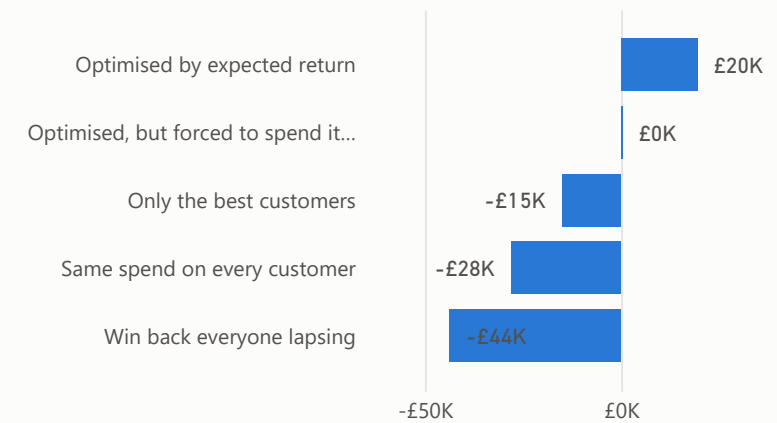
Profit by plan, median across 2,000 assumption runs
