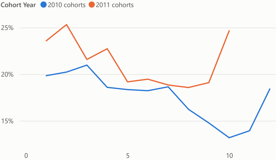
First year retention, 2010 vs 2011 cohorts
