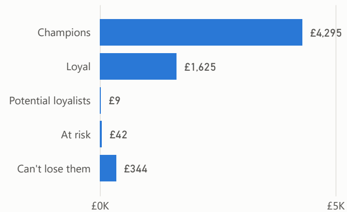
Planned spend by segment
