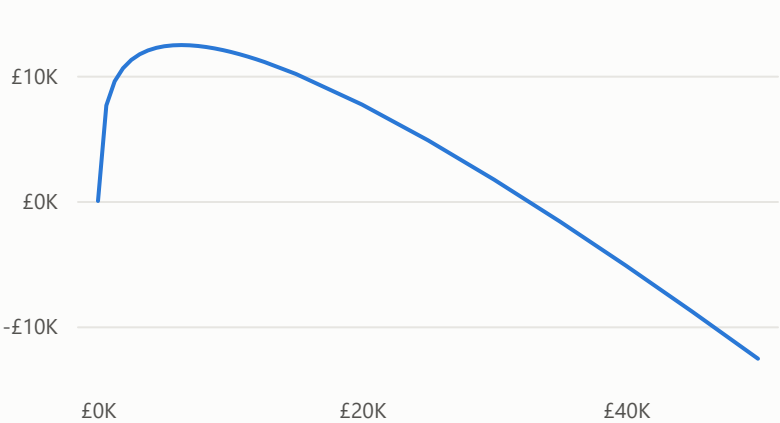
Profit after spend at each budget (best placement)
