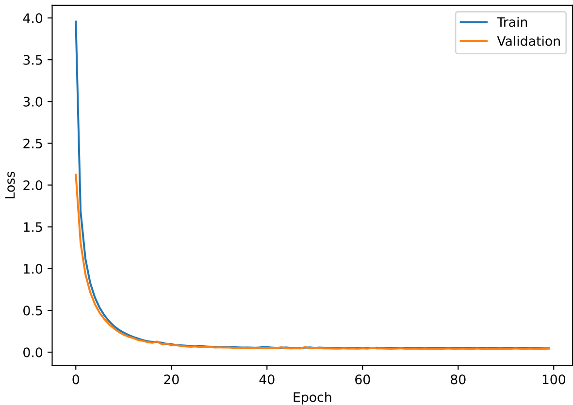
Model loss
