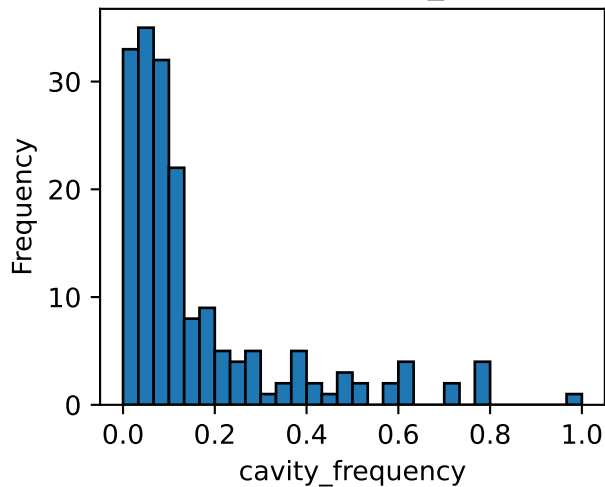
Validation Set cavity_frequency
