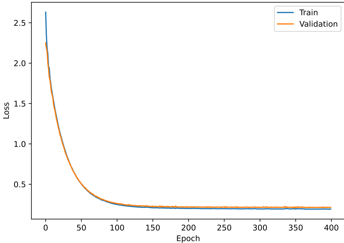
Model loss
