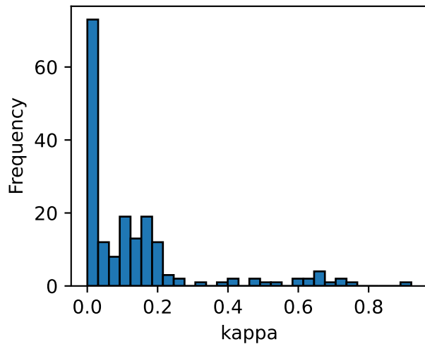
Validation Set kappa
