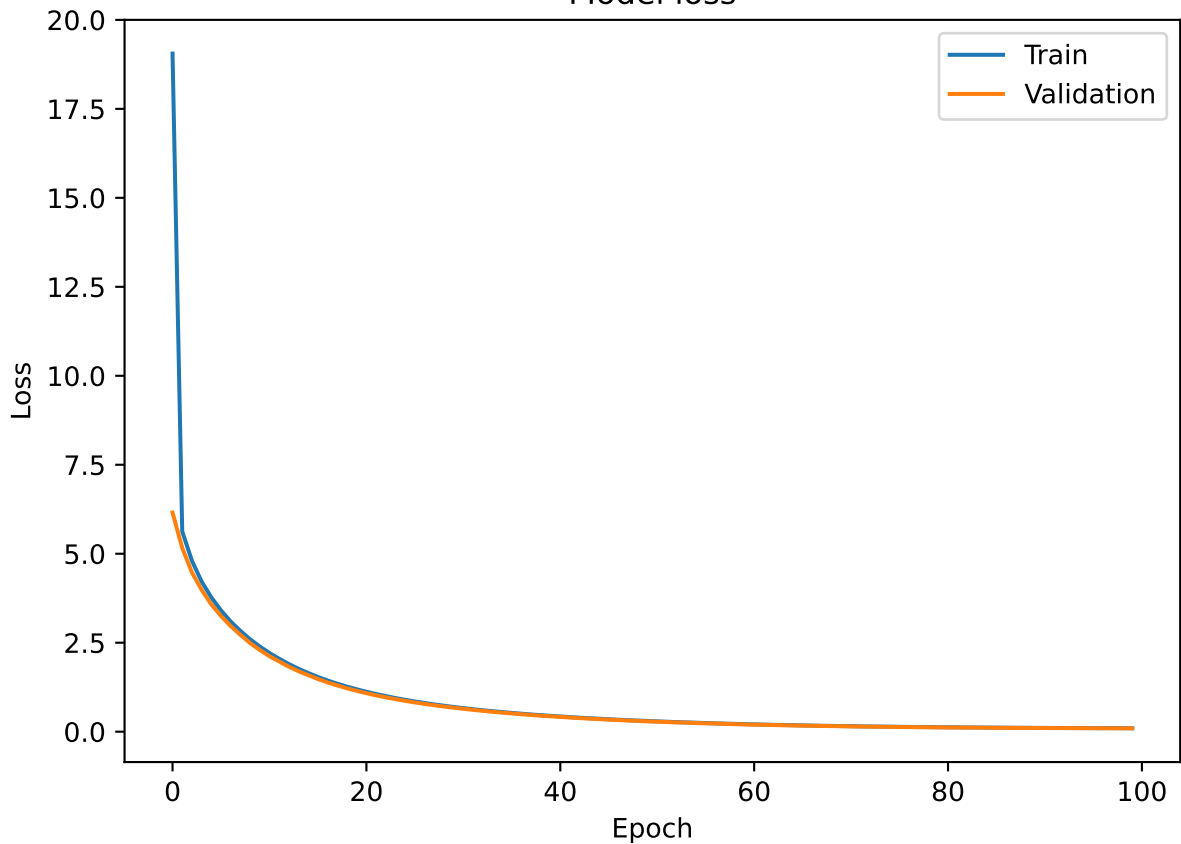
Model loss
