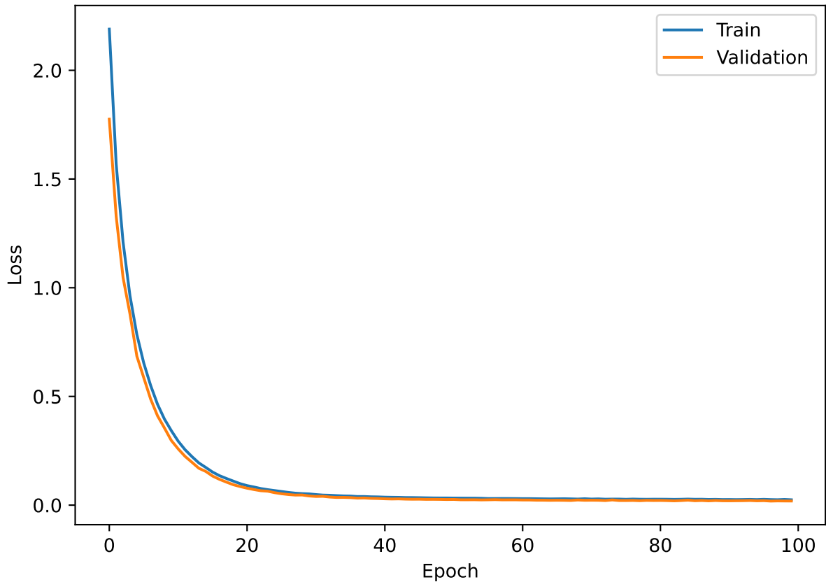
Model loss
