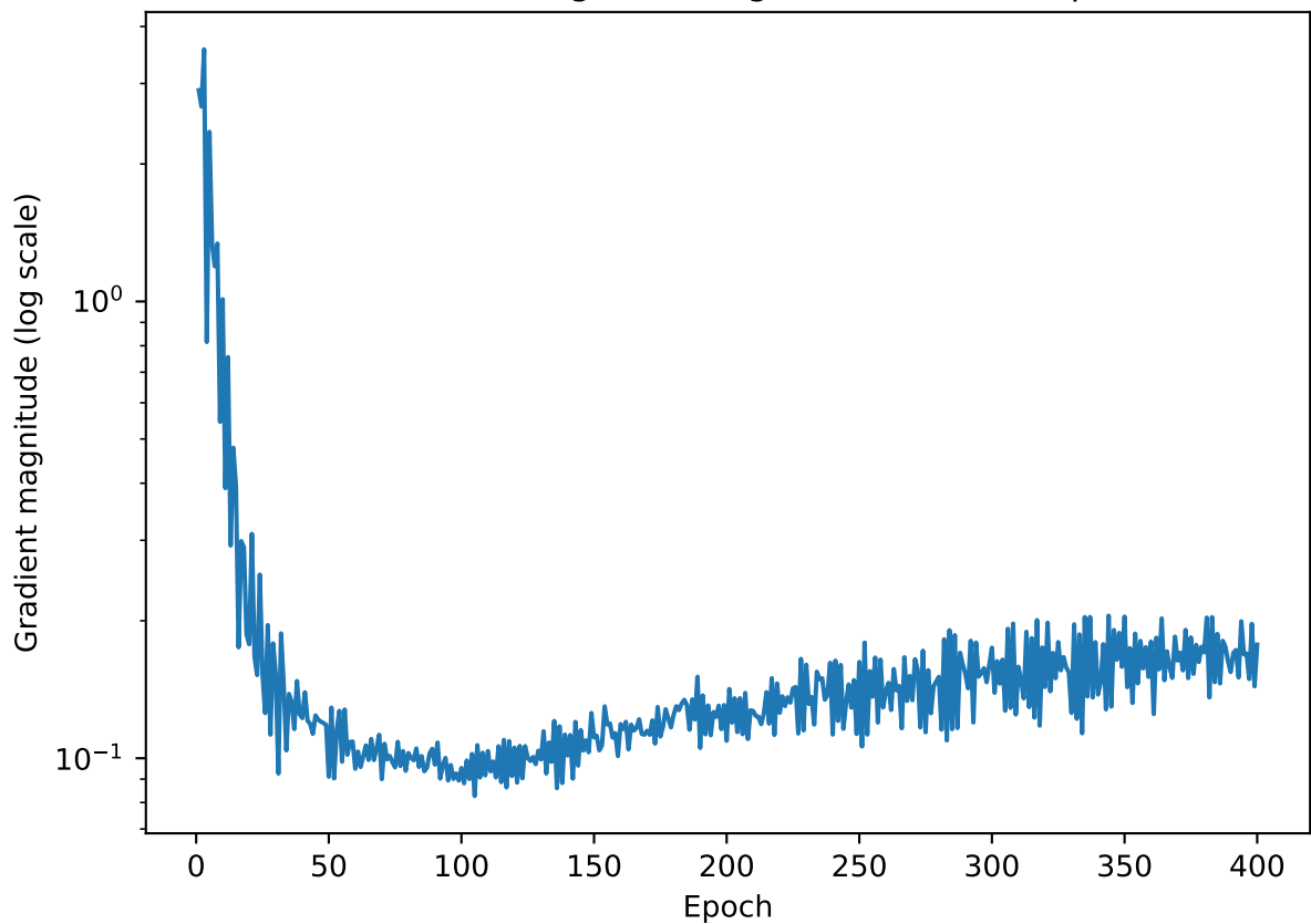
Gradient tracking for a single batch across epochs
