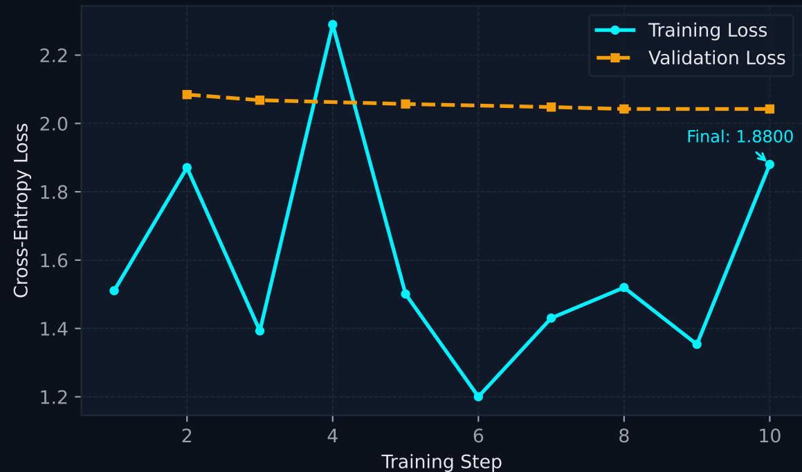
Figure 1 — LoRA Fine-Tuning Loss Convergence
