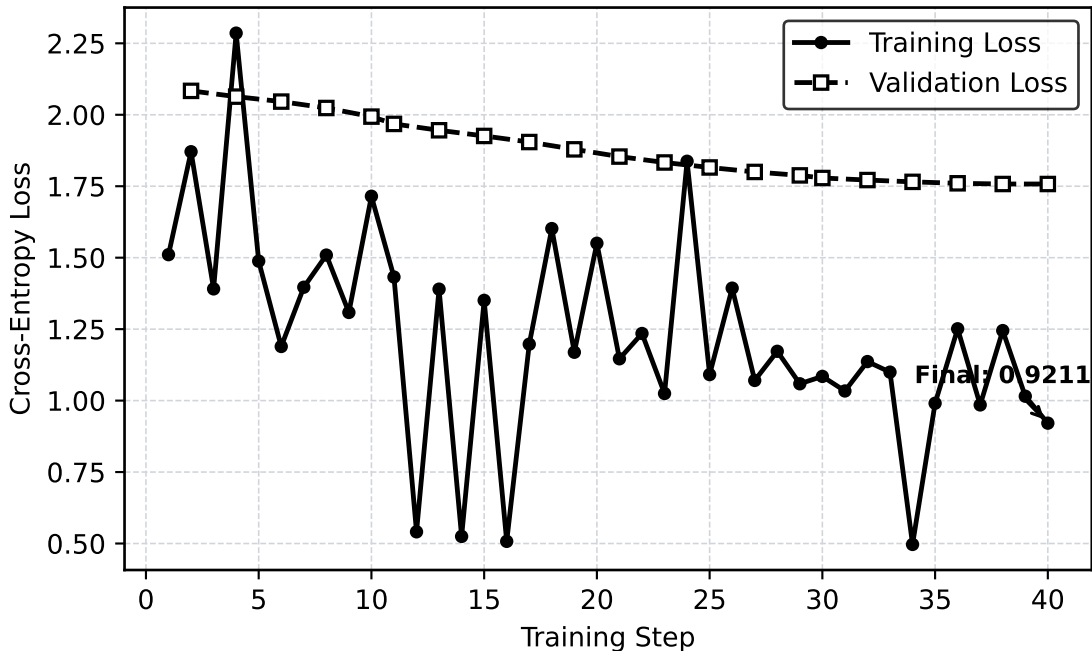
Figure 1 — LoRA Fine-Tuning Loss Convergence
