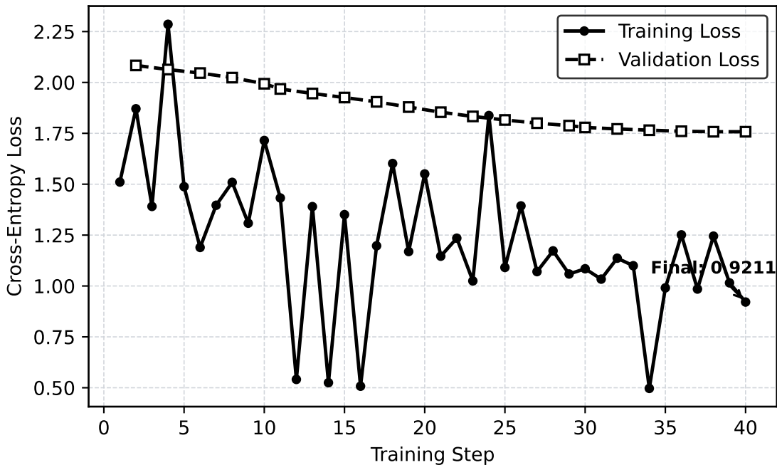
LoRA Fine-Tuning Loss Convergence
