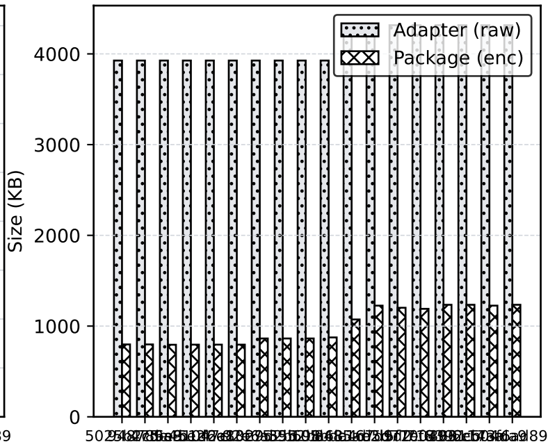
Adapter vs Encrypted Package Size
