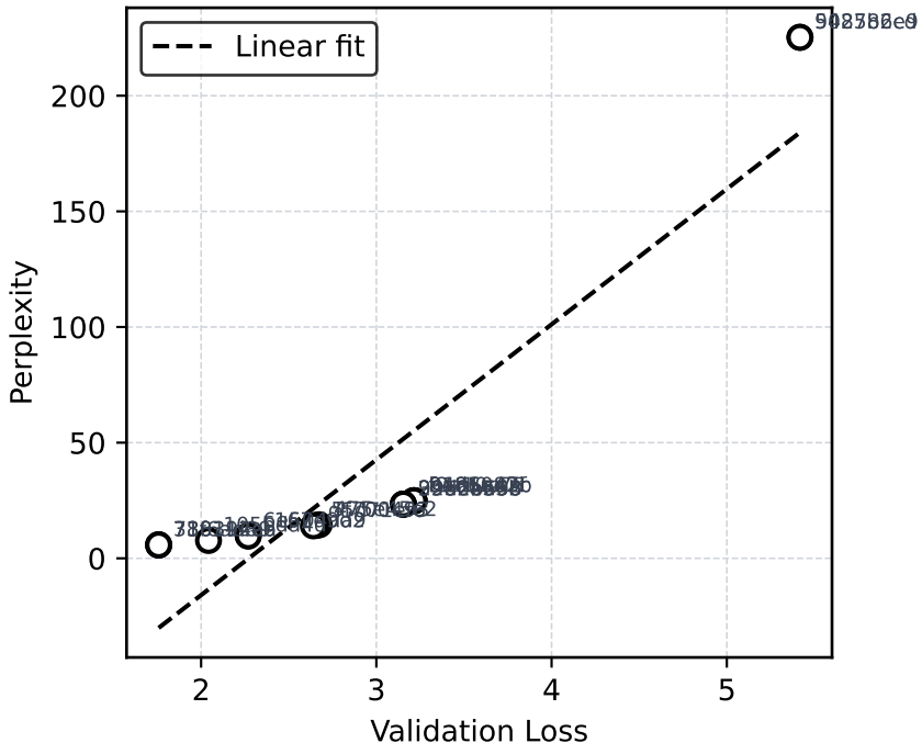
Perplexity vs Validation Loss
