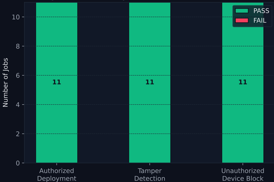
Figure 4 — Security Gate Pass/Fail Across All Jobs
