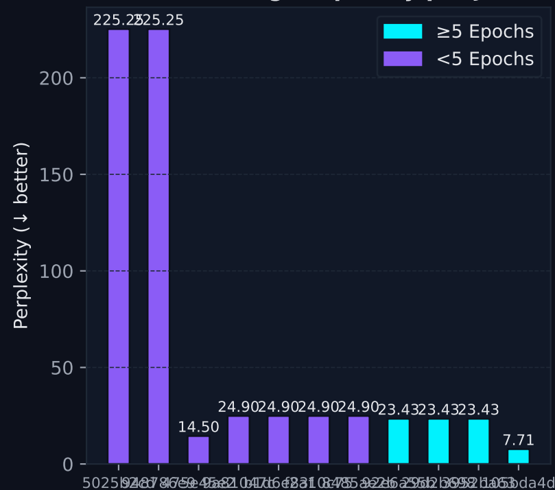
Post-Training Perplexity per Job
